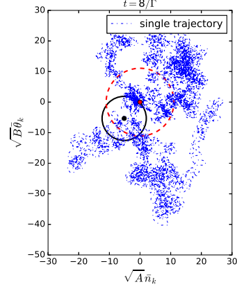
FIG. 3. Evolution of the phase-space distribution for a single trajectory from time t = 0 to t = 8/\Gamma in absence of feedback. The mode k = 0.1\sqrt{mg\bar{\rho}}/\hbar is considered, with the initial temperature T_i = 1.1g\bar{\rho} and a loss rate \Gamma = \omega_k/400 . Scattered blue points give the evolution of the center R . We verified that C_{12} stays small while, at any time, A_k C_{11} \simeq B_k C_{22} \simeq E_c/2 , as expected for such a large \omega_k . The black solid-circle, of radius \sqrt{E_c} , represents the final RMS width of the Wigner function. For comparison, the red dashed-circle, of radius \sqrt{E} , where E is the energy obtained after averaging over 100 trajectories, gives the rms width of the averaged phase space distribution. The coordinates are given in the frame rotating according to the free evolution: namely, the plotted quantity is \tilde{R} = (\tilde{n}_k, \tilde{\theta}_k) = \mathfrak{R}^{-1}(\omega_k t)R .
