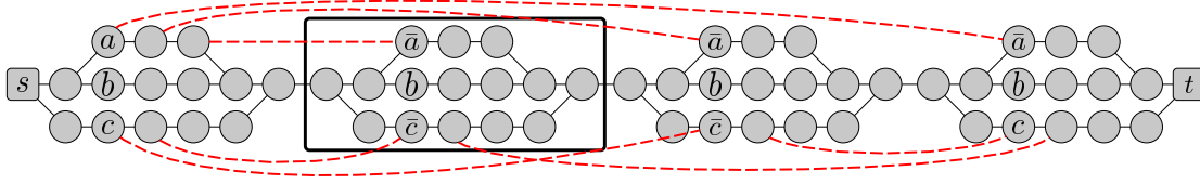
Fig. 9: Graph equivalent to the 3-SAT formula (a \vee b \vee c) \wedge (\bar{a} \vee b \vee \bar{c}) \wedge (\bar{a} \vee b \vee \bar{c}) \wedge (\bar{a} \vee b \vee c) . Vertices of M are squares. In the black rectangle, gadget corresponding to the clause (\bar{a} \vee b \vee \bar{c}) . The dashed edges denote conflicts.
