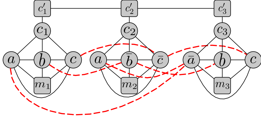
Figure 10: Graph equivalent to the 3-SAT formula (a \vee b \vee c) \wedge (a \vee \bar{b} \vee \bar{c}) \wedge (\bar{a} \vee b \vee c) . Vertices of M are squares. The dashed edges denote conflicts.
