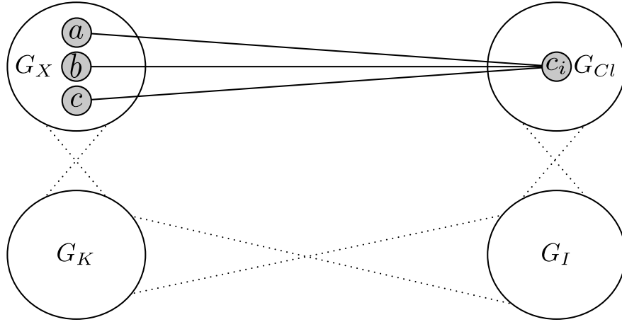
Figure 7: Construction of the dense graph. Dotted lines represent complete bipartites between subsets of vertices.
