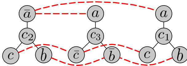
Figure 3: Graph equivalent to the 3-SAT formula (\bar{a} \vee b \vee c) \wedge (a \vee \bar{b} \vee \bar{c}) \wedge (a \vee b \vee c) . The dashed edges denote conflicts.
