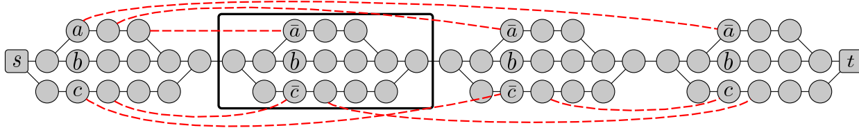
Figure 9: Graph equivalent to the 3-SAT formula (a \vee b \vee c) \wedge (\bar{a} \vee b \vee \bar{c}) \wedge (\bar{a} \vee b \vee \bar{c}) \wedge (\bar{a} \vee b \vee c) . Vertices of M are squares. In the black rectangle, gadget corresponding to the clause (\bar{a} \vee b \vee \bar{c}) . The dashed edges denote conflicts.
