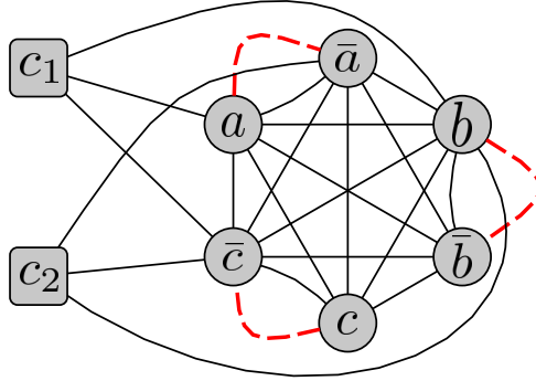
Figure 11: Graph equivalent to the 3-SAT formula (a \vee \bar{c} \vee b) \wedge (\bar{a} \vee b \vee \bar{c}) . Vertices of M are squares. The dashed edges denote conflicts.
