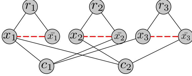
Figure 2: Reduction from the 3-SAT instance (x_1 \vee \bar{x}_2 \vee x_3) \wedge (x_1 \vee x_2 \vee \bar{x}_3) to an instance of TDSwnC. The dashed edges denote conflicts.
