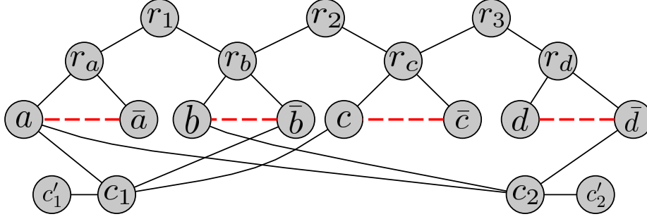
Figure 6: Graph equivalent to the 3-SAT formula (a \vee \bar{b} \vee c) \wedge (a \vee b \vee \bar{d}) . The dashed edges denote conflicts.
