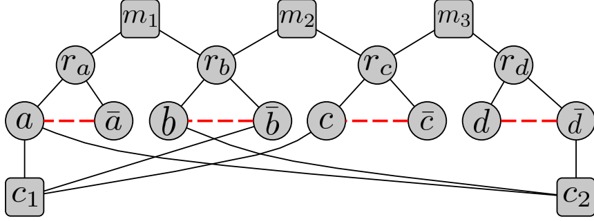
Figure 8: Graph equivalent to the 3-SAT formula (a \vee \bar{b} \vee c) \wedge (a \vee b \vee \bar{d}) . Vertices of M are squares. The dashed edges denote conflicts.
