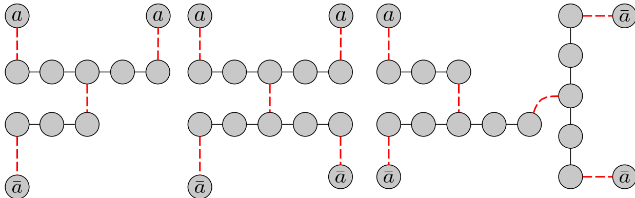
Figure 4: Gadget used to split K_{1,2} (left), K_{2,2} (middle) and K_{1,3} (right) of conflicts into graphs of maximum degree 1. The dashed edges denote conflicts.
