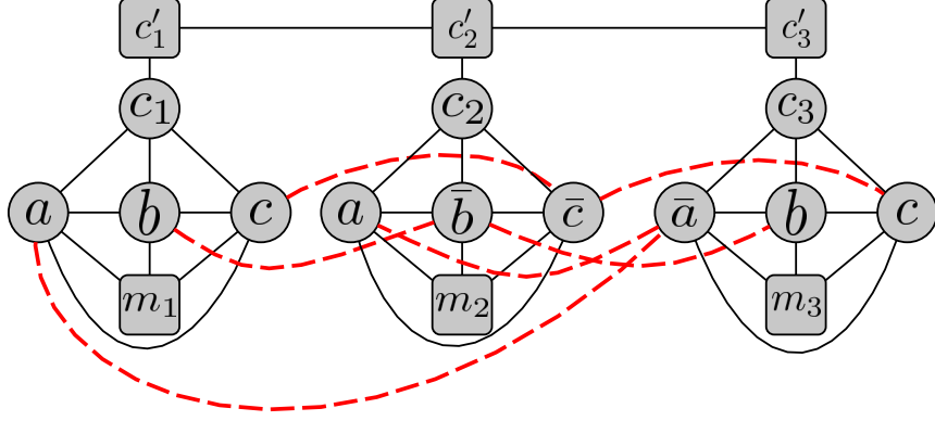
Figure 10: Graph equivalent to the 3 SAT formula (a \vee b \vee c) \wedge (a \vee \bar{b} \vee \bar{c}) \wedge (\bar{a} \vee b \vee c) . Vertices of M are squares.
