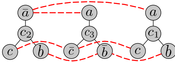
Figure 3: Graph equivalent to the 3 SAT formula (\bar{a} \vee b \vee c) \wedge (a \vee \bar{b} \vee \bar{c}) \wedge (a \vee b \vee c)
