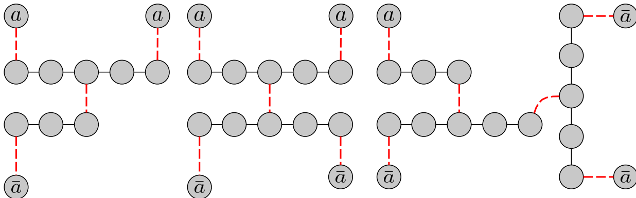
Figure 4: Gadget used to split K_{1,2} (left), K_{2,2} (middle) and K_{1,3} (right) of conflict into graphs of maximum degree 1
