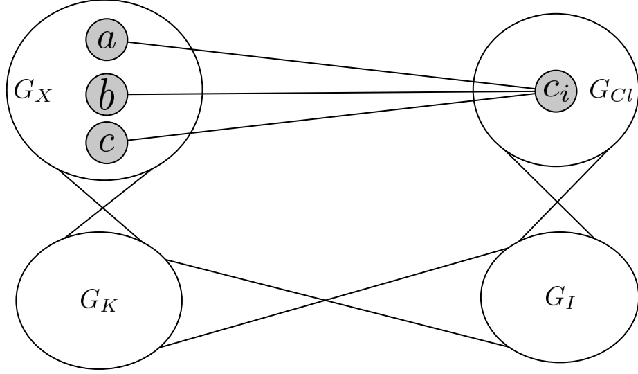
Figure 7: Construction of the dense graph
