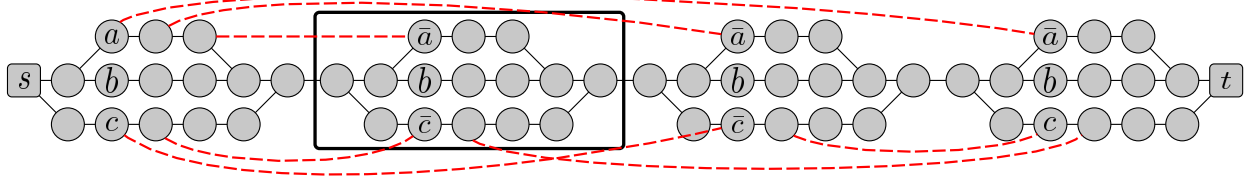
Figure 9: Graph equivalent to the 3 SAT formula (a \vee b \vee c) \wedge (\bar{a} \vee b \vee \bar{c}) \wedge (\bar{a} \vee b \vee \bar{c}) \wedge (\bar{a} \vee b \vee c) . Vertices of M are squares. In the black rectangle, gadget corresponding to the clause (\bar{a} \vee b \vee \bar{c}) .
