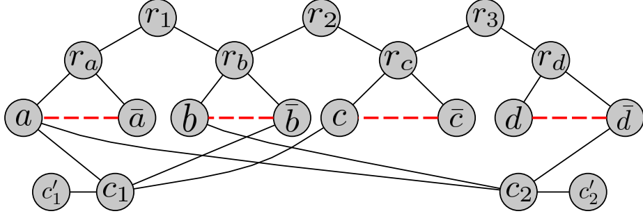
Figure 6: Graph equivalent to the 3 SAT formula (a \vee \bar{b} \vee c) \wedge (a \vee b \vee \bar{d})
