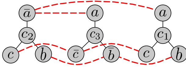
Figure 3: Graph equivalent to the 3 SAT formula (\bar{a} \vee b \vee c) \wedge (a \vee \bar{b} \vee \bar{c}) \wedge (a \vee b \vee c)
