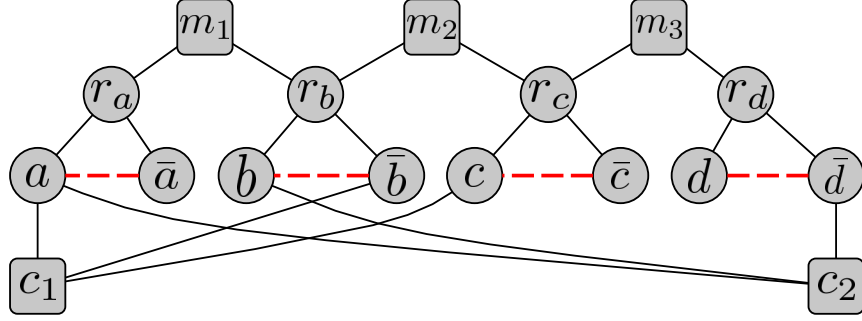
Figure 8: Graph equivalent to the 3 SAT formula (a \vee \bar{b} \vee c) \wedge (a \vee b \vee \bar{d}) . Vertices of M are squares.
