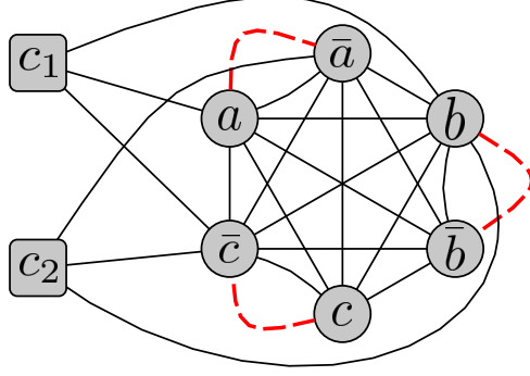
Figure 11: Graph equivalent to the 3 SAT formula (a \vee \bar{c} \vee b) \wedge (\bar{a} \vee b \vee \bar{c}) . Vertices of M are squares.
