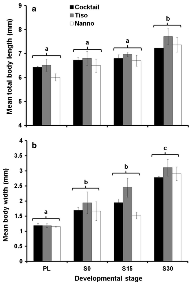
Fig. 2 Growth performance of Pseudopleuronectes americanus during development and according to diet: a total body length and b maximum body width in mm (mean \pm SE) by developmental stage (PL pelagic larvae; S0 at settlement; S15 15 days after settlement; and S30 30 days after settlement). Developmental groups not sharing a common letter are significantly different (two-way ANOVA; P < 0.05 )
