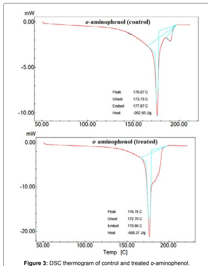
Figure 3: DSC thermogram of control and treated o -aminophenol.
