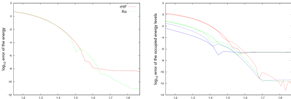
Figure 2 – Log-log plot of the error on the total energy (left) and the three occupied energy levels (right) of the carbon atom for the rHF (solid lines) and X\alpha (dashed lines) models as a function of the mesh size N_I , for a fixed cut-off radius L_e = 50 (the reference calculation corresponds to L_e = 100 and N_I = 100 ).
