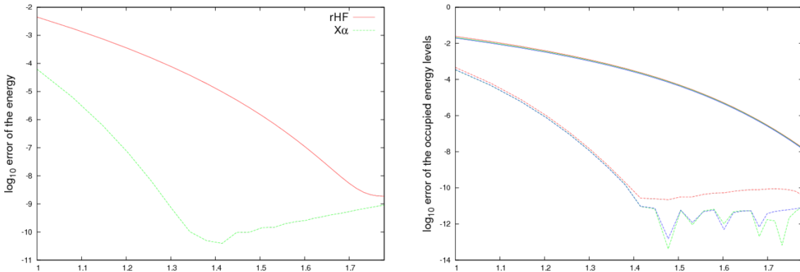
Figure 1 – Log-log plot of the error on the total energy (left) and the three occupied energy levels (right) of the carbon atom for the rHF (solid lines) and X\alpha (dashed lines) models as a function of the cut-off radius L_e for a fixed mesh size N_I = 50 (the reference calculation corresponds to L_e = 100 and N_I = 100 ).
