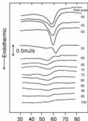
Fig. 20.15 DSC heating curves of 5% aqueous dispersions of curdlan after heating at various temperatures for 60 min. Heating rate: 1^{\circ}\text{C min}^{-1} . The number beside each curve represent the temperature in ^{\circ}\text{C} at which the dispersion was kept. 41
