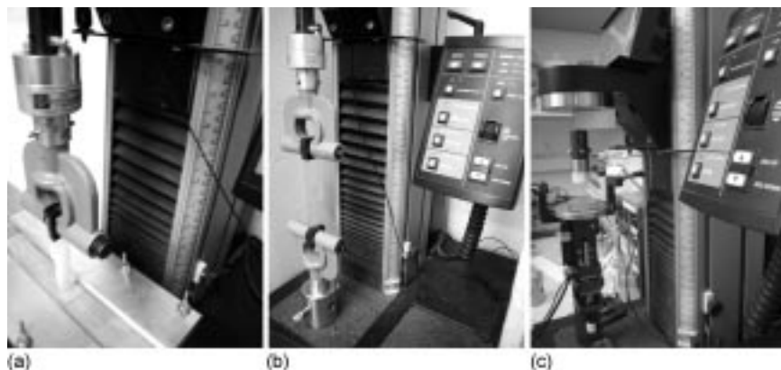
Fig. 28.3 (a) Specimen mounted on the Instron Universal Testing Machine (UTM) during the 90^\circ peel test. (b) Specimen mounted on the Instron UTM prior to application of the lap-shear test. (c) A modified probe-tack test in which a special device is capable of detecting the first contact between the probe and a pressure-sensitive adhesive (PSA) and determining this contact as the initial dwell time.
