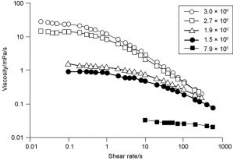
Fig. 1.5 Viscosity–shear rate profiles for 1% solutions of guar gum of varying molecular mass.
