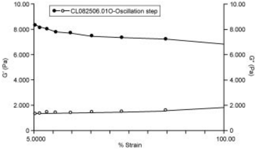
Fig. 27.2 Strain sweep curve for traditional MCC/CMC.
