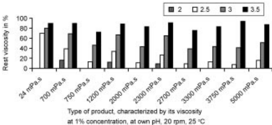
Fig. 10.10 Acid stability of different guar solutions at certain pHs prepared at 86–89 °C for 10 minutes, while stirring, expressed as rest viscosity in %, based on viscosity at pH 4 times 100%.
