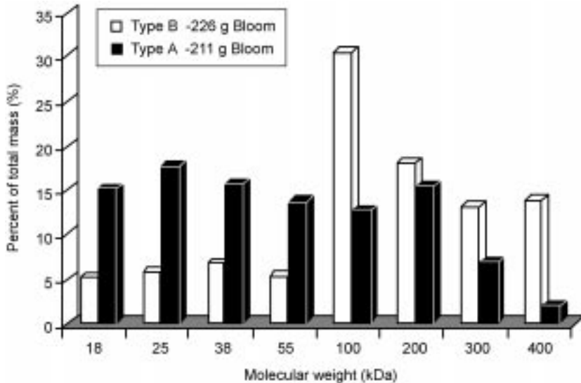
Fig. 6.3 The molecular weight distribution for two gelatins with similar Bloom values (Product information, DGF Stoes, 1999). The type A gelatin has an average molecular weight of 94 kDa and a viscosity of 2.5 mPas (6.67%, 60 °C). The type B gelatin has an average M_w of 171 kDa while the viscosity is 5.9 mPas (6.67%, 60 °C).
