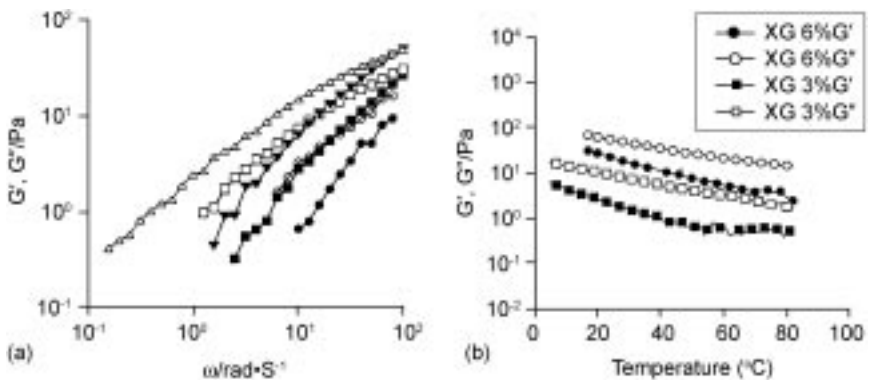
Fig. 19.6 (a) Frequency dependence of G' and G'' for dispersions of xyloglucan with various concentrations at 5°C. Strain, 0.05. Concentration of xyloglucan, ●, 1.05 wt% G' ; ○, 1.05 wt% G'' ; ■, 1.40 wt% G' ; □, 1.40 wt% G'' ; ▼, 1.75 wt% G' ; △, 1.75 wt% G'' . (b) Temperature dependence of G' and G'' for 3.0 and 6.0 wt% dispersions of xyloglucan. Heating rate, 1°C/min. Angular freq, 1 rad/s, strain, 0.05.
