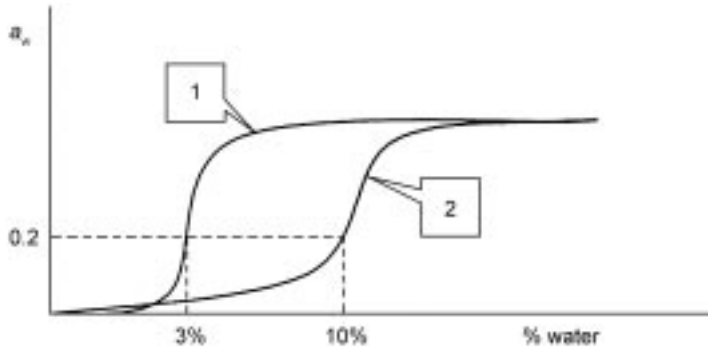
Fig. 30.9 Absorption profiles.
