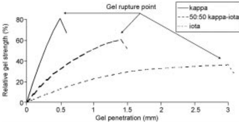
Fig. 7.7 Gel properties of pure and blended kappa and iota carrageenans.
