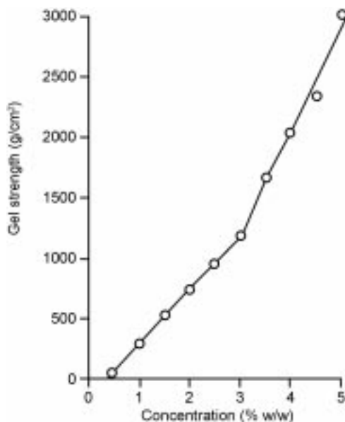
Fig. 20.7 Concentration dependence of gel strength for curdlan at 30 °C (curdlan gel was obtained by heating at 90 °C for 10 min).
