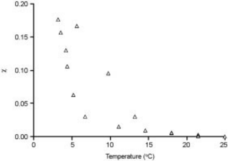
Fig. 6.4 Helix amount ( \chi ) in 2(w/v)% cold water fish gelatin solution cooled and heated at a rate of 0.5°C/min in the temperature range 25°–4°–25°C (Haug, 2003).
