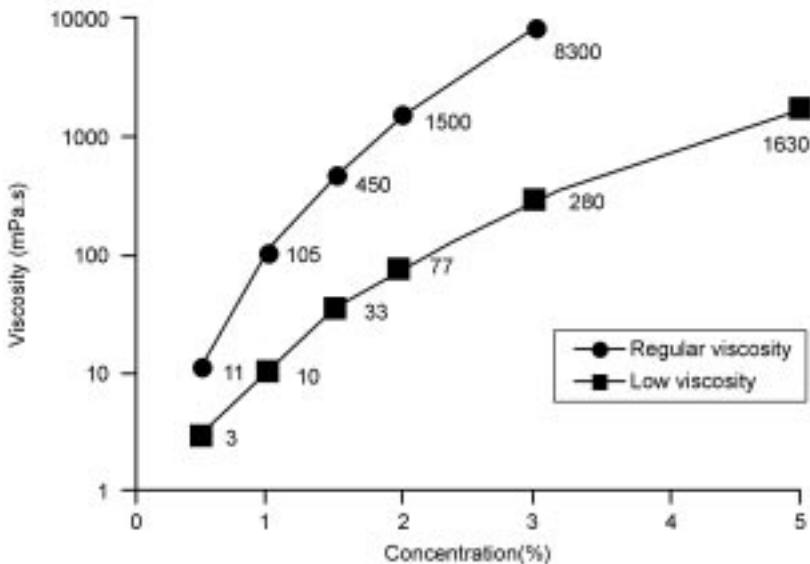
Fig. 19.14 Concentration dependence of steady shear viscosity of TSX and LVTSX at 25°C and at a shear rate of 8.6 \text{ s}^{-1} .
