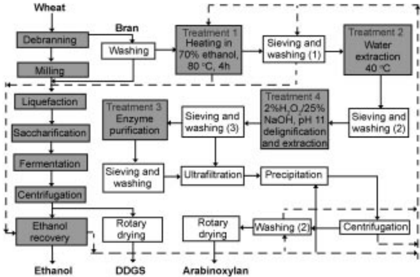
Fig. 23.3 Integrated processes for ethanol and arabinoxylan co-production from wheat. Adapted from Sadhukhan et al. (2008).
