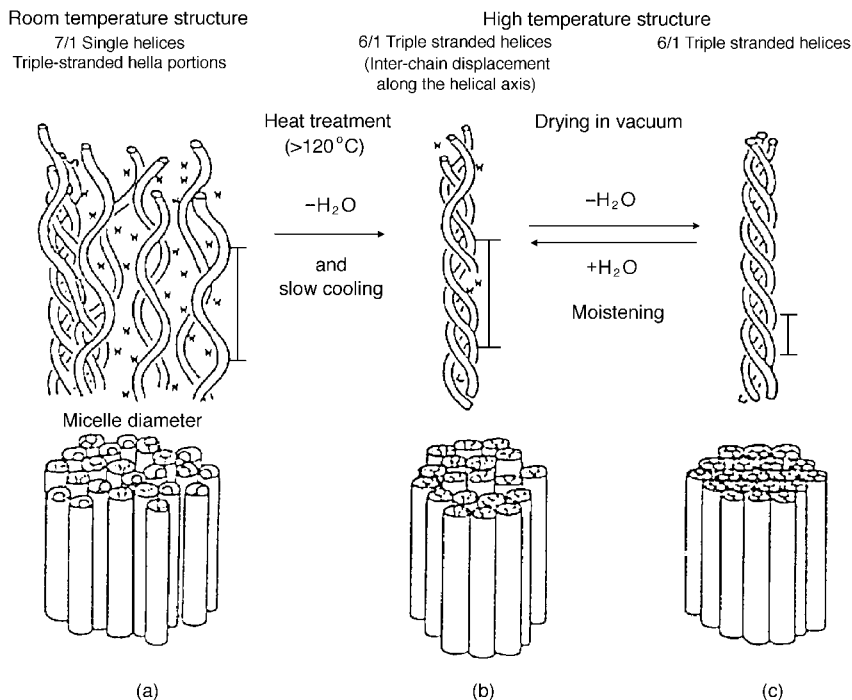
Fig. 20.13 Schematic representation of structural change between three forms of curdlan: (a) room temperature structure; (b) high temperature structure at high humidity; (c) high temperature structure at low humidity. 31
