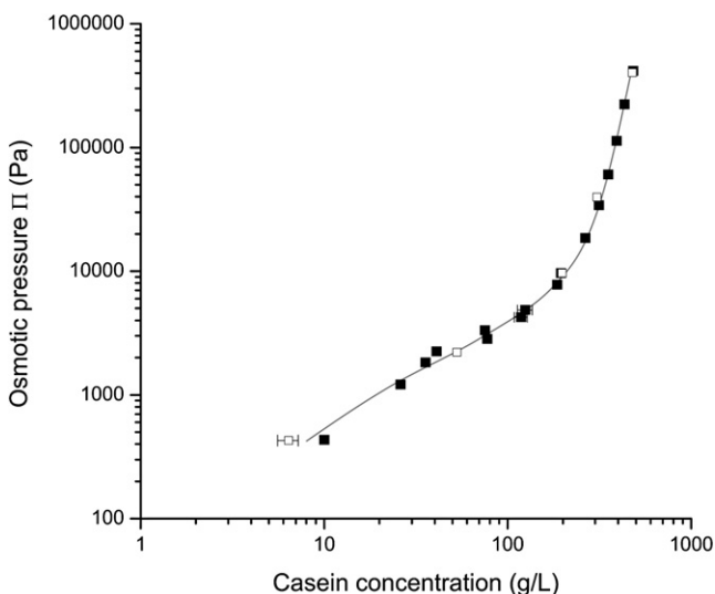
FIGURE 2 Osmotic pressures of casein micelle dispersions: NPC powder 1 in UF permeate (solid squares); NPC powder 2 in UF permeate (open squares). Vertical scale: osmotic pressure of the stressing solution, in Pa. Horizontal scale, casein concentration within the dialysis bag. The solid line is a guide for the eye.
