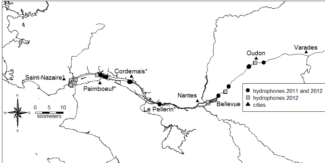
Telemetry array in the Loire Estuary (from Tétard et al. In press)
