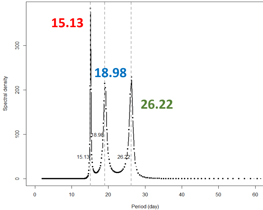
Spectral density for the distance travelled in 2011. The three main rhythms are highlighted in grey (15.13, 18.98 and 26.22 days) (from Tétard et al. in press)
