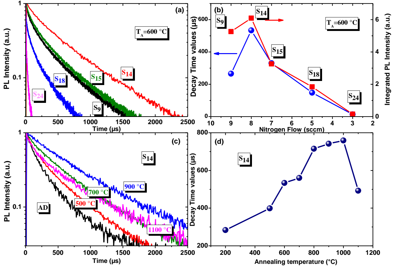
Figure 9. At the 545 nm ( {}^5D_4 \rightarrow {}^7F_3 ) wavelength (a) the normalized decay curves for samples S 9 to S 24 annealed at T_A=600 °C and (b) their corresponding decay time with the evolution of the integrated PL intensity (c) the PL decay curves for the optimized layer S 14 annealed at the indicative T_A and (d) their corresponding decay time.
