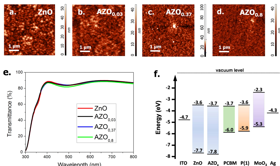
Figure 1. Atomic force microscopy (AFM) images ( 5 \mu\text{m} \times 5 \mu\text{m} ) recorded in tapping mode of ZnO (a), \text{AZO}_{0.03} (b), \text{AZO}_{0.37} (c), and \text{AZO}_{0.8} (d) deposited on glass/ITO substrates. Their surface roughness (RMS) is 8, 6, 4, and 4 nm, respectively. Transmittance spectra (e) of ZnO (red), \text{AZO}_{0.03} (black), \text{AZO}_{0.37} (blue), and \text{AZO}_{0.8} (green) films deposited on glass/ITO substrates. Energy level diagram of the materials employed in the solar cells (f).
