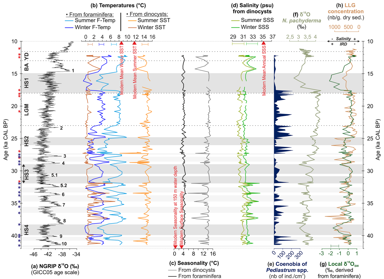
Figure 3. Reconstructed hydrological parameters derived from dinocyst and planktonic foraminifera assemblages compared to (a) NGRIP-GIICC05 \delta^{18}\text{O} record: (b) temperatures, (c) seasonality (mean summer minus mean winter temperatures), (d) SSS derived from dinocysts, (e) Abundances of coenobia of the freshwater algae Pediastrum spp., (f) \delta^{18}\text{O} measured on N. pachyderma , (g) local \delta^{18}\text{O}_{\text{sw}} derived from \delta^{18}\text{O} on N. pachyderma , and (h) large lithic grain (LLG) concentration, plotted on a reverse scale. Stars, bands, DO number and acronyms: same legend as Fig. 2.
