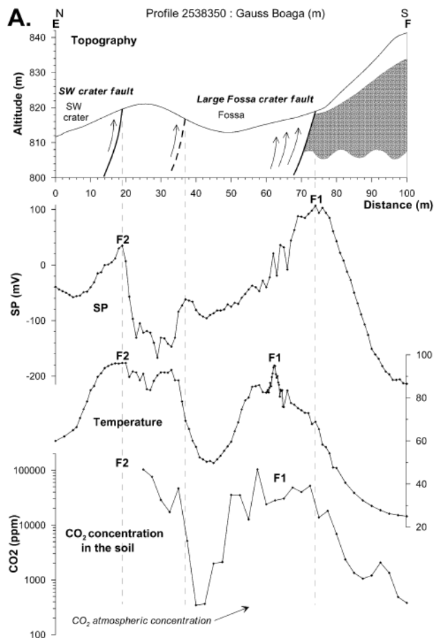
Fig. 8 A CO 2 , T, SP and topographical E–F profile located in the detailed study area shown in Fig. 2. The name of the profile corresponds to the easting co-ordinates. F1, F2, etc. correspond to the anomalies shown on the maps. B GHIJ profile shown in Fig. 2
