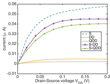
Figure 4: Current-Voltage characteristics obtained with the five different models.
