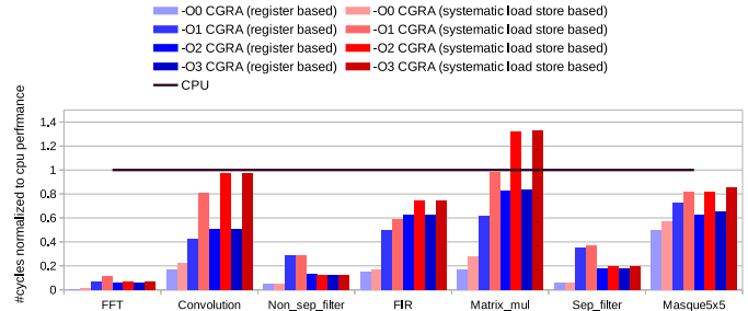
Fig. 6. Performance of proposed mapping approach in a CGRA with infinite band-width
