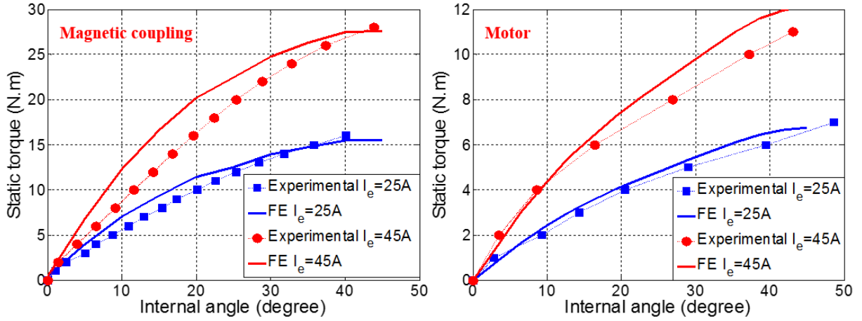
Figure 16 Static torque measured for inductor currents I_e = 25 A and 45 A , left: magnetic coupling, right: motor.
