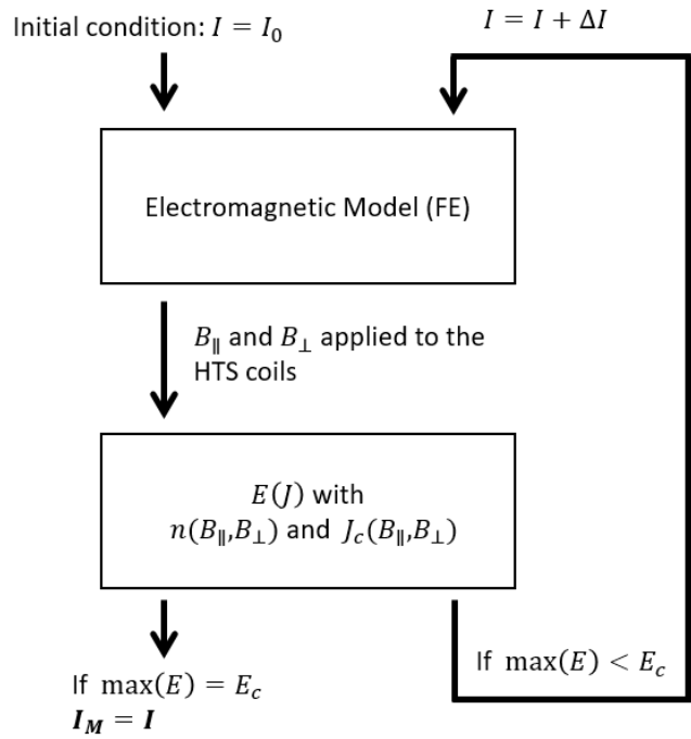
Figure 6 Method for the operating current determination of the HTS coils.
