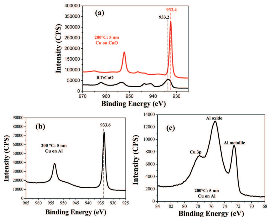
Figure 4. (a) Cu 2p core level spectra from CuO and after 5 nm Cu deposition (at 10 °C) and annealing to 200 °C, (b) Cu 2p core level spectra from 5nm Cu deposition (at -140 °C) on Al and after annealing to 200 °C, and (c) Al 2p core level spectra from 5 nm Cu deposition (at -140 °C) on Al and after annealing to 200 °C.
