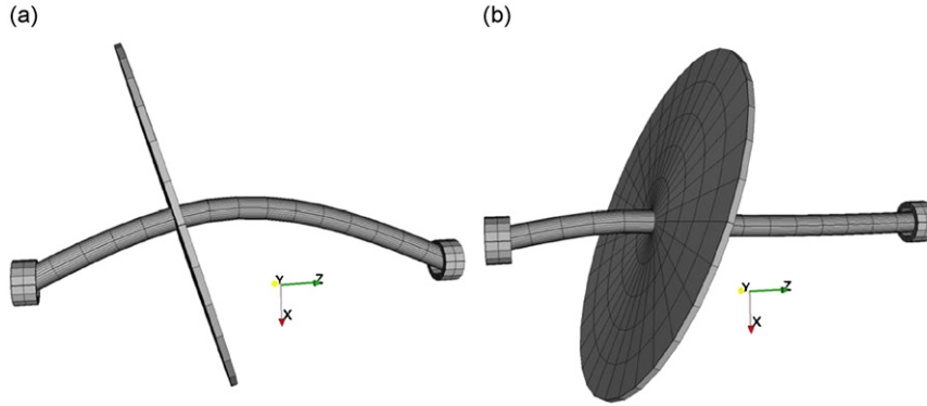
Fig. 10. Eigenmodes of a 3D model of a disc on a flexible shaft: (a) Global bending mode ( \omega_{\text{bending}} = 628 \text{ rad/s} ). (b) Second eigenmode with disc flexibility ( \omega_{\text{disc}} = 974 \text{ rad/s} ).
