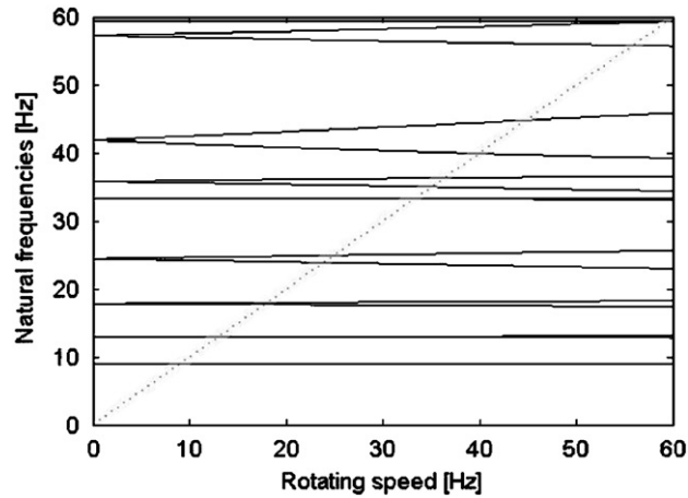
Fig. 17. Evolution of the natural frequencies in the inertial frame. Natural frequencies in full line. Synchronous whirl in dashed line.
