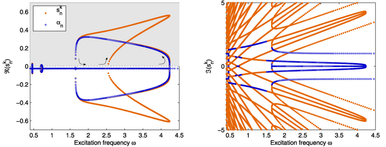
Fig. 3. Eigenvalues of \mathbf{H} as a function of the excitation frequency \omega , corresponding to the simulation of Fig. 1. ‘•’: all s_n^k , for n = 1, 2 and k = 0, \pm 1, \dots, \pm H ; ‘o’: \alpha_n , n = 1, 2 computed with the Hill’s method. (left): real part; (right): imaginary part. Gray region corresponds to unstable periodic solutions.
