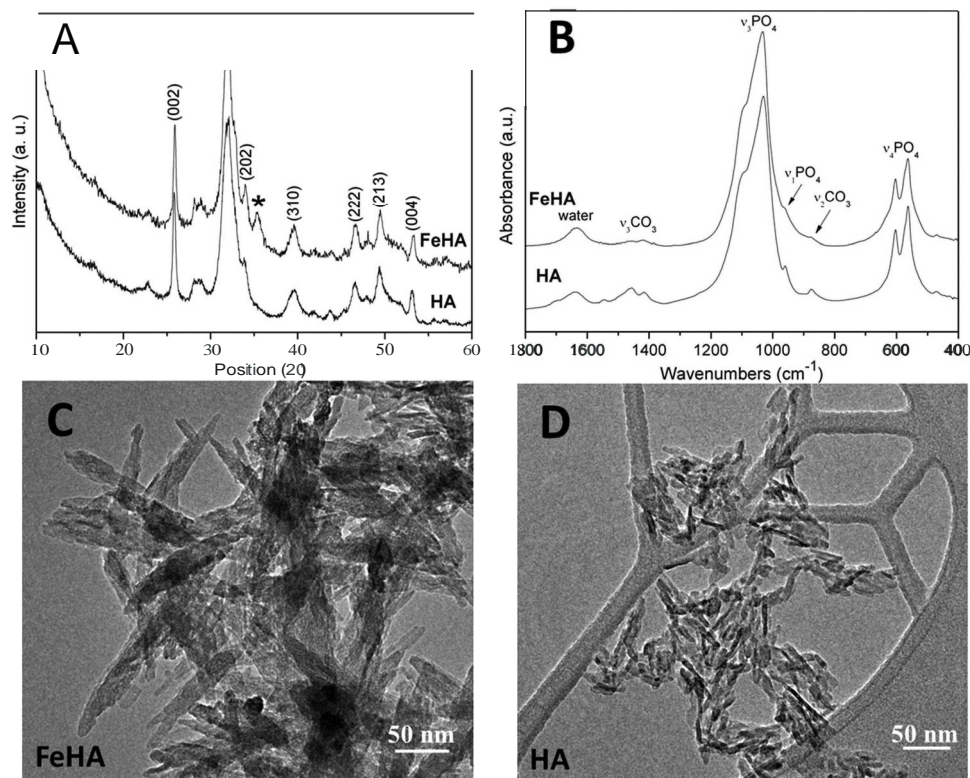
Fig. 1 (A) XRD spectra, (B) FTIR spectra and (C and D) TEM images of FeHA and HA NPs.
