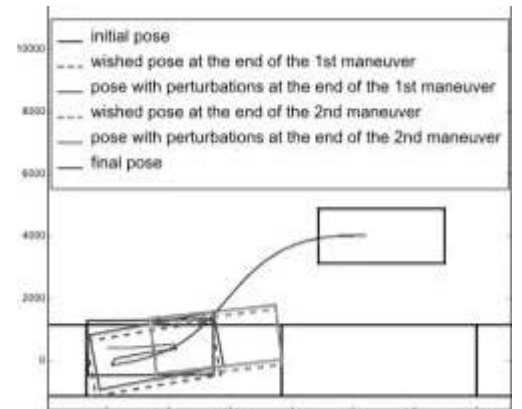
Fig. 13 Parking with perturbations without regeneration
