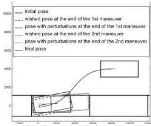
Fig. 14 Parking with perturbations with regeneration
