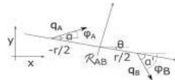
Fig. 8 Frames involved in bi-elementary paths
