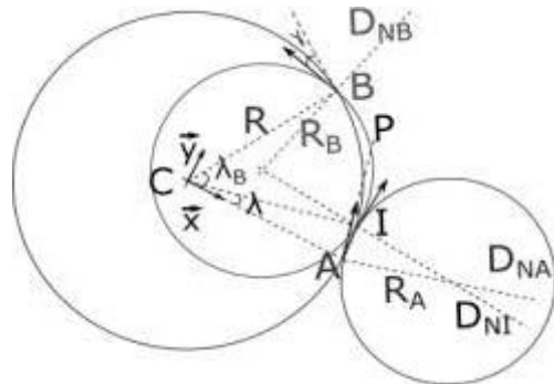
Fig. 11 Solution based on two circle arcs
