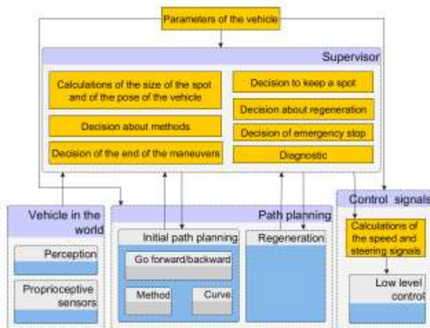
Fig. 15 Global functional architecture
