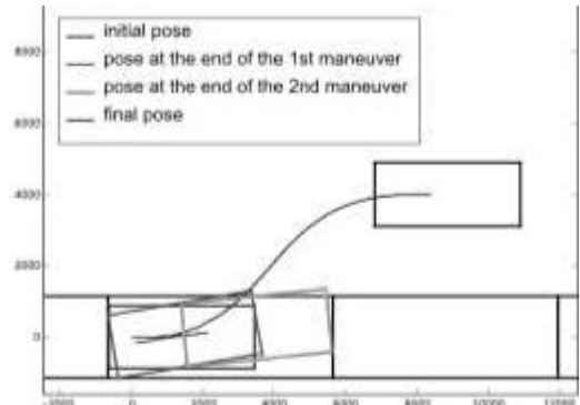
Fig. 12 Perfect parking in 3 maneuvers
