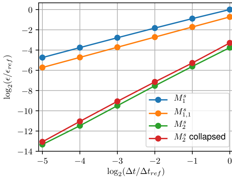
FIGURE 5.1. Time order convergence for the 2D Euler gravity test case with D2Q9 model. Convergence is estimated using the relative L^2 error \epsilon on macroscopic variables with respect to the analytical solution at t_{max} \approx 0.12 . The reference values (\Delta t_{ref}, \epsilon_{ref}) of the logarithmic scale are \Delta t_{ref} = 0.024 , \epsilon_{ref} = 0.0143 .
