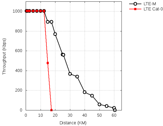
Fig. 3. Throughput variation with Distance
