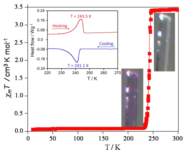
Figure 1. Thermal dependence of the \chi_m T product recorded at 0.4 \text{ K.mn}^{-1} in a settle mode, DSC study recorded at 2 \text{ K.mn}^{-1} (inset), and crystal images in the LS and HS states showing the clear thermochromism from purple to colourless, respectively.
