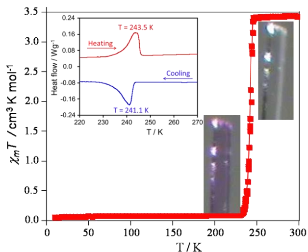
Figure 1. Thermal dependence of the \chi_m T product recorded at 0.4 \text{ K}\cdot\text{mn}^{-1} in a settle mode, DSC study recorded at 2 \text{ K}\cdot\text{mn}^{-1} (inset), and crystal images in the LS and HS states showing the clear thermochromism from purple to colourless, respectively.
