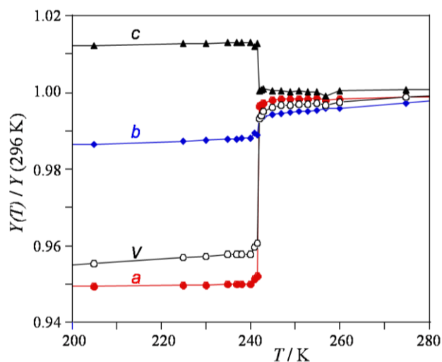
Figure 3. Thermal evolution of the lattice parameters ( a , b , c ) and unit cell volume for 1 , showing the anisotropic changes (expansion along a , b and contraction along c axis) upon SCO transition.
