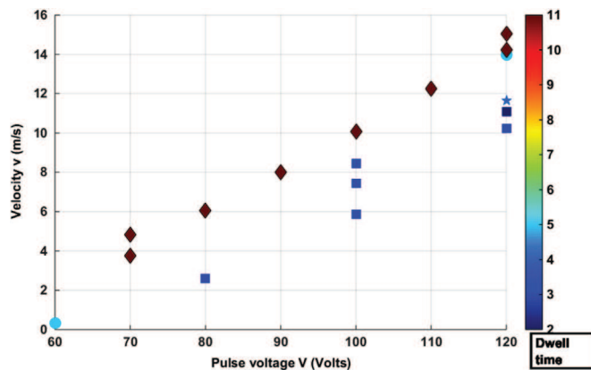
Fig. 17. Filament growth rate v_0 as a function of peak voltage V , for the Silica 2 ink. Each symbol corresponds to a different dwell time, also indicated on the colorbar. As seems to lead to a larger end velocity. An affine relation v_{end} = \beta(V - V_{min}) can be fitted to the data. (For interpretation of the references to colour in this figure caption, the reader is referred to the web version of this paper.)
