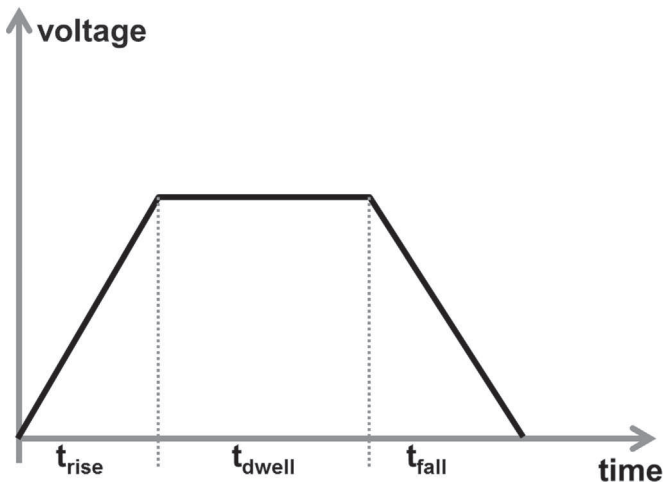
Fig. 2. Schematic of the actuation pulse for the nozzle. The voltage increases during t_{rise} , then stays at a fixed value during t_{dwell} , and then decreases to zero during t_{fall} . The duration of each segment of the waveform can be selected independently, but the total time cannot exceed 15 \mu s .
