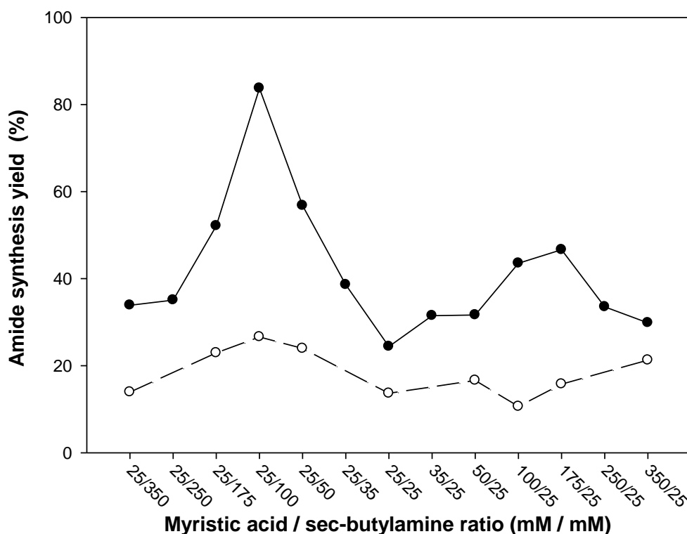
Fig 3. Effect of the myristic acid/ sec -butylamine molar ratio on the equilibrium amide synthesis yield. Reactions were carried out in tert -amyl alcohol using (R)- sec -butylamine (●) or (S)- sec -butylamine (○) for 48 hours at 55°C with 50 g.l -1 of Candida antarctica lipase B.
