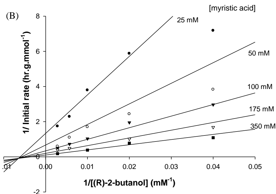
Fig. 2. Reciprocal initial rates versus reciprocal substrate concentrations. The synthesis was carried out at 55°C using 10 g.l -1 of Candida antarctica lipase B. (A) The concentration of (R)-2-butan-2-ol was fixed at 25 mM (●), 50 mM (○), 100 mM (▼), 175 mM (▽) and 350 mM (■). (B) The concentration of myristic acid was fixed at 25 mM (●), 50 mM (○), 100 mM (▼), 175 mM (▽) and 350 mM (■). The data represent the averages of triplicate runs whose standard deviations were always lower than 15%.
