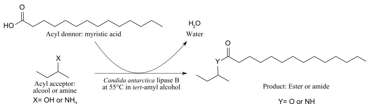
Scheme 1. Acylation of monofunctional alcohols and amines catalyzed by C. antarctica lipase B in tert -amyl alcohol.
