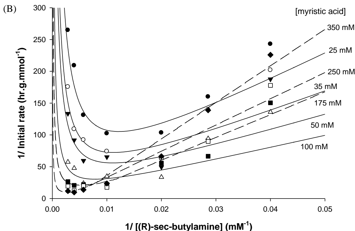
Fig. 4. Reciprocal initial rates versus reciprocal substrate concentrations. The synthesis was carried out at 55°C using 50 g.L -1 of Candida antarctica lipase B. (A) Myristic acid concentration was varied from 25 to 350 mM and (R)-sec-butylamine concentration was fixed at 25 mM (●), 35 mM (○), 50 mM (▼), 100 mM (△), 175 mM (■), 250 mM (□) and 350 mM (◆). (B) (R)-sec-butylamine concentration was varied from 25 to 350 mM and myristic acid concentration was fixed at 25 mM (●), 35 mM (○), 50 mM (▼), 100 mM (△), 175 mM (■), 250 mM (□) and 350 mM (◆). The data represent the averages of triplicate runs whose standard deviations were always lower than 15%.
