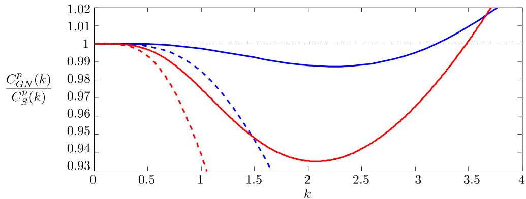
Linear phase velocity errors
