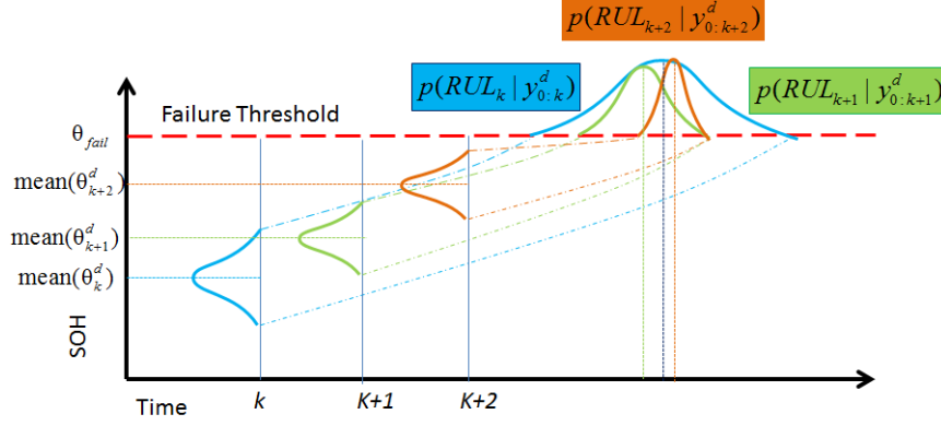
Fig. 7.3 Schematic illustration of RUL prediction process
