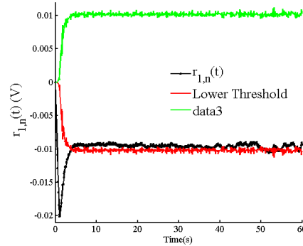
Fig. 7.11 Residual r_1(t) under nominal conditions
