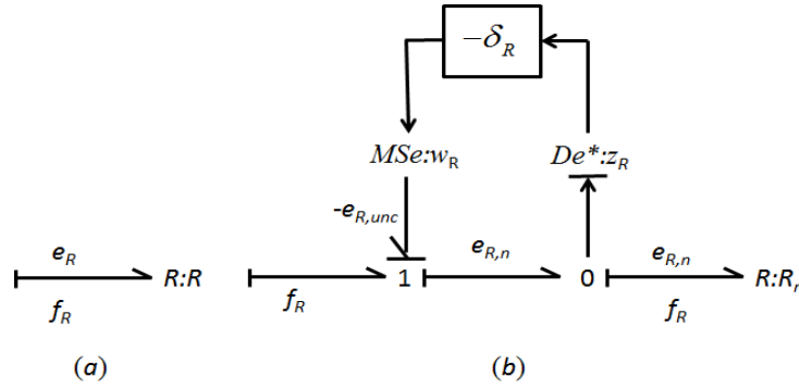
Fig. 7.1 R-element in resistance causality. (b): uncertain R-element in resistance causality in LFT form.
