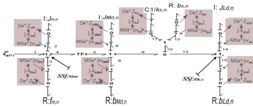
Fig. 7.10 BG-LFT Model of monitorable part of the system
