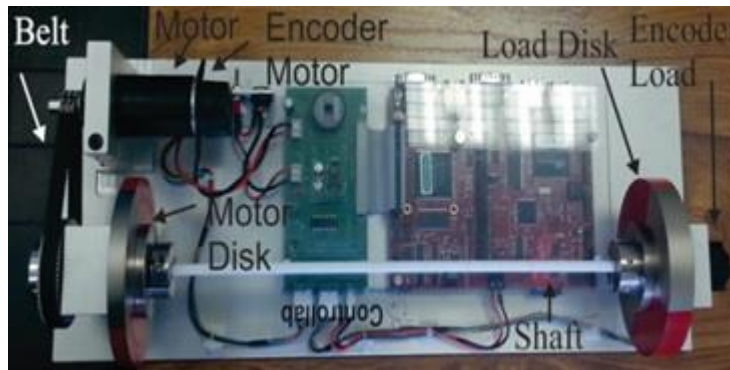
Fig.7.6 Mechatronic torsion bar 1.0 system
