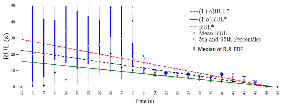
Fig. 7.17 RUL Predictions
