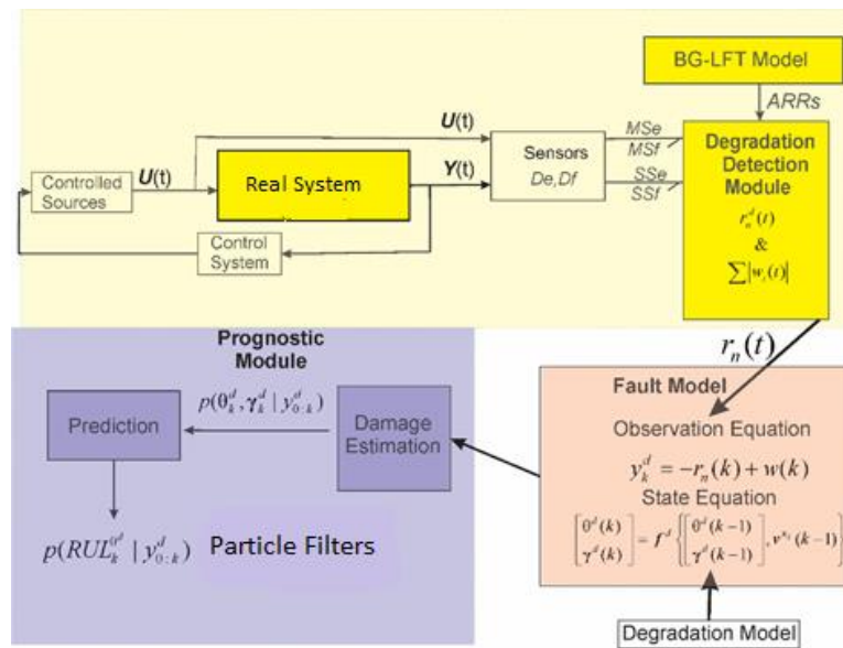
Fig. 7.4 Schematic description of the Health Monitoring Methodology
