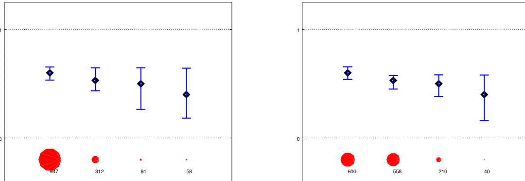
FIGURE 2. Number of draws of the KLUCB (right) and Track-and-Stop (left) algorithms on one run of length t = 1408 (the stopping time of Track-and-Stop). Confidence intervals on the unknown mean of each arm (black diamond) are also displayed.
