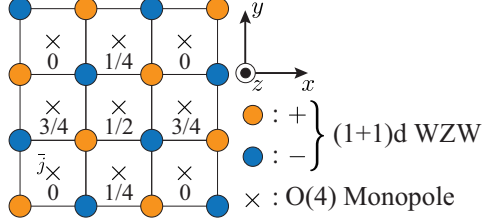
FIG. 4: (Color online) A top view (from the +z direction) of a staggered array of (1+1)d O(4) NL\sigma models with a WZ term, each running in the z direction. In a precise analogy with the 2d counterpart discussed in Sec. III, the staggered summation over the WZ terms is converted into a collection of monopole Berry phases. As in the 2d case, the weights \zeta_{\bar{j}} = 0, 1/4, 1/2, 3/4 are assigned to the monopoles occurring at the dual sites \{\bar{j}\} .
