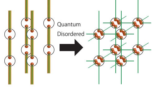
FIG. 5: (Color online) Thick orange lines depict an array of (1+1)d O(4) NL\sigma models with WZ terms at level k_{\text{eff}} = 4S/3 , which are placed in the background of a prefixed VBS_z order (green lines) - see text for details. Condensation of monopoles results in a 3d AKLT-like state on the cubic lattice.
