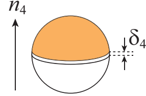
FIG. 3: (Color online) The modified topological charge Q_{\tau xy} for the case n_4 = \delta_4 . The sphere shown schematically is S^3 . The topological charge is given by the shaded area ( = \int_0^{\arccos \delta_4} 4\pi \sin^2 \theta d\theta ) divided by \text{vol}(S^3) = 2\pi^2 .
