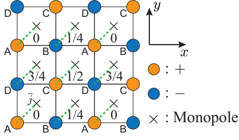
FIG. 2: (Color online) The spatial distribution of the weight Y_{\bar{j}} entering (via eq.(13)) the Berry phases associated with monopoles residing on the dual sites \bar{j} (i.e., the center of the plaquettes of the direct lattice). Each plaquette is assigned a sublattice index (A, B, C, D) coinciding with that of the vertex to the southwest of the center (dashed lines).
