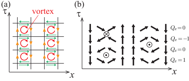
FIG. 1: (Color online) (a) The rewriting, following Ref. 40 , of the staggered summation over planar spin Berry phases (3) into the net space-time vorticity (4). The directions of the vertical arrows on the temporal links account for the staggering of the Berry phases. Each arrow contributes to the action the piece iS(-1)^j \Delta_\tau \phi . The auxiliary horizontal arrows on the spatial links stand for \pm iS \Delta_x \phi . (b) An illustration depicting how space-time vortices induce a discontinuous jump (i.e., a phase slip) in the winding number (9) associated with the snapshot configuration.
