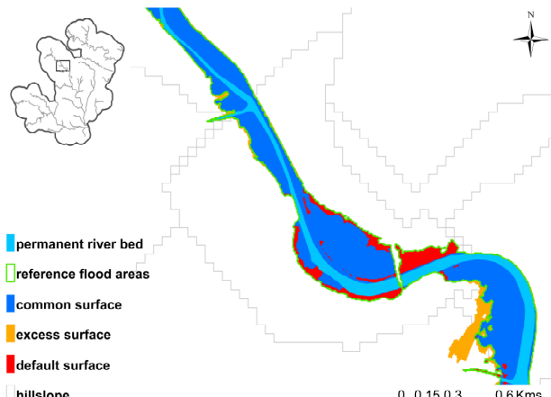
Figure 5. Illustration of comparison between estimated and reference inundated areas: definition of common surface ( Sc ), excess surface ( Se ), and default surface ( Sd ).
