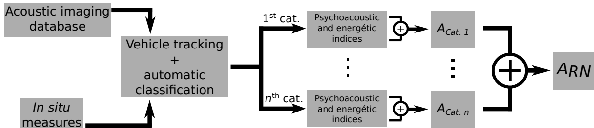
Figure 7 – Schematic diagram of adapting the model Morel et al. [10] with the data coming from the Megamicros system. With A_{RN} the total road traffic annoyance et A_{cat.n} the specific annoyance of the n^{th} vehicle category.
