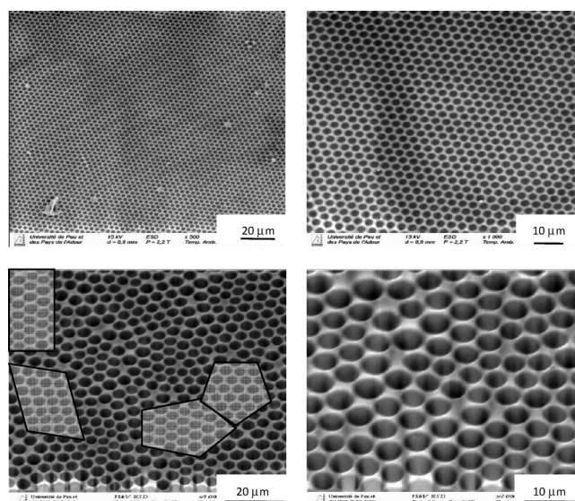
Figure 5. SEM images of HC structured film obtained with \text{PS-COO}^{-}\text{Na}^{+} (top) and BF patterned film with \text{PS-COOH} (bottom) from C_p = 10 \text{ g L}^{-1} over mica at room temperature under hood air flow and 85% of humidity (left and right scale bars are 20 and 10 \mu\text{m} , respectively).
