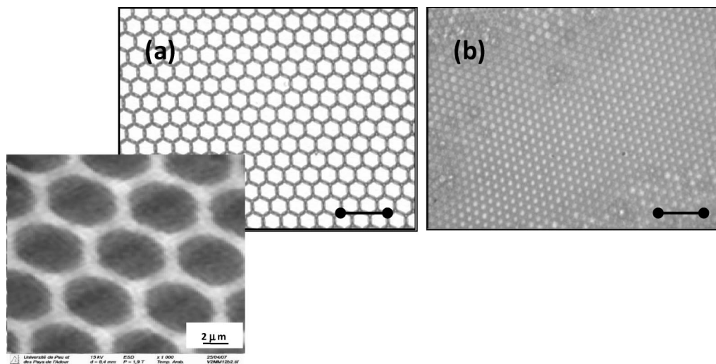
Figure 4. SEM image (scale bar = 2 \mu\text{m} ) and optical micrographs of polystyrene honeycomb structures on mica substrate with different polymer solution concentrations C_p = (a) 1.2 and (b) 10 \text{g L}^{-1} (scale bar = 20 \mu\text{m} ).
