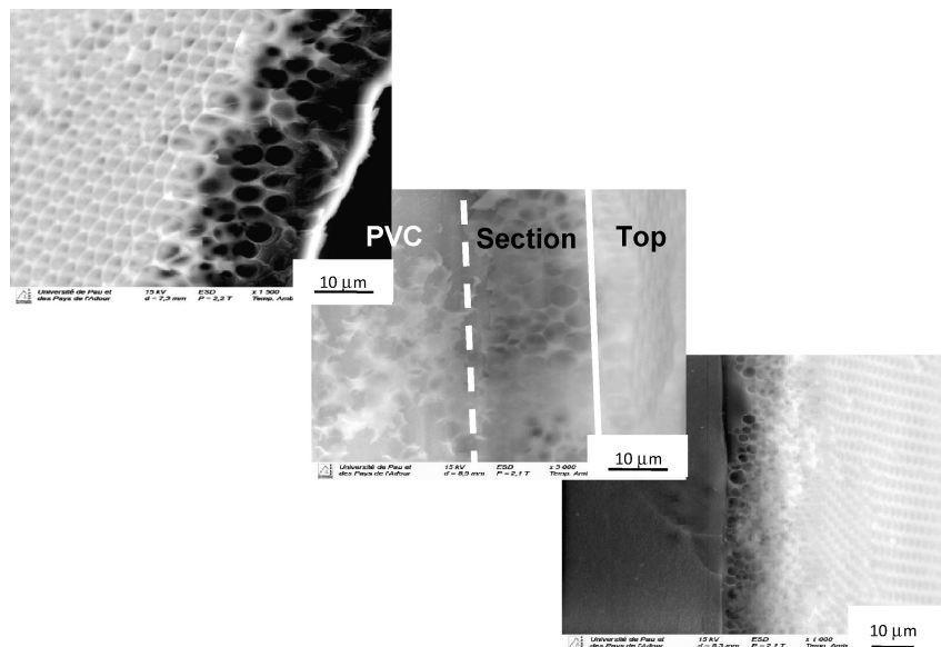
Figure 7. SEM images of cross section of polystyrene honeycomb structured film on mica, PVC sheet, and PMMA plate, from a polymer solution concentration C_p = 10 \text{ g L}^{-1} (from top to bottom, respectively) (scale bar = 10 \mu\text{m} ).
