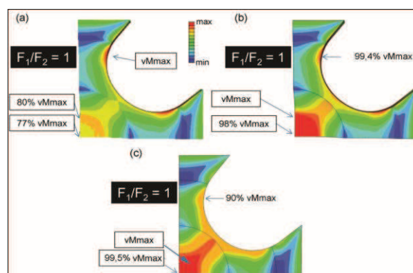
Fig. 2 Visualization of the von Mises stress field for an equibiaxial loading of 95 kN applied to three different designs. (a) Initial design with a central thickness of 1.6mm; (b) Second design with a reduced thickness of
