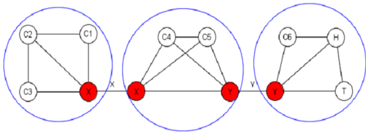
Figure 3: Decomposing result of symbol graph of T_{fam} with minimal separator S^* = \{X\} and S^{*' } = \{Y\}
