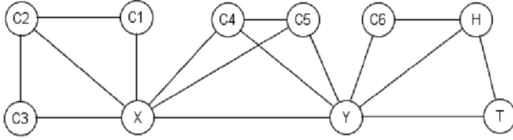
Figure 2: Symbol graph presenting TBox T_{fam}
