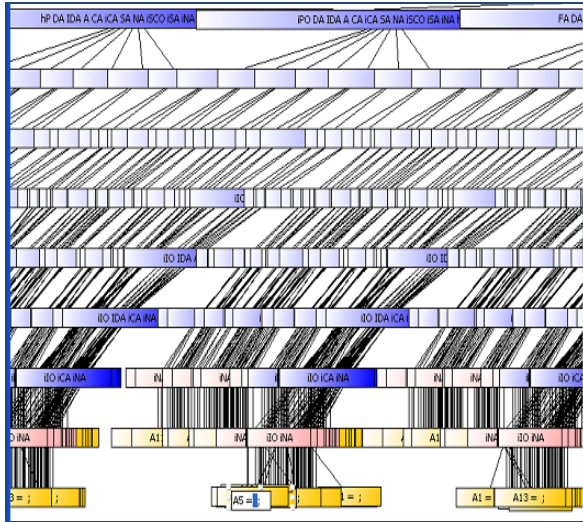
Figure 6: decomposition graph based on minimal separator of Tambis1
