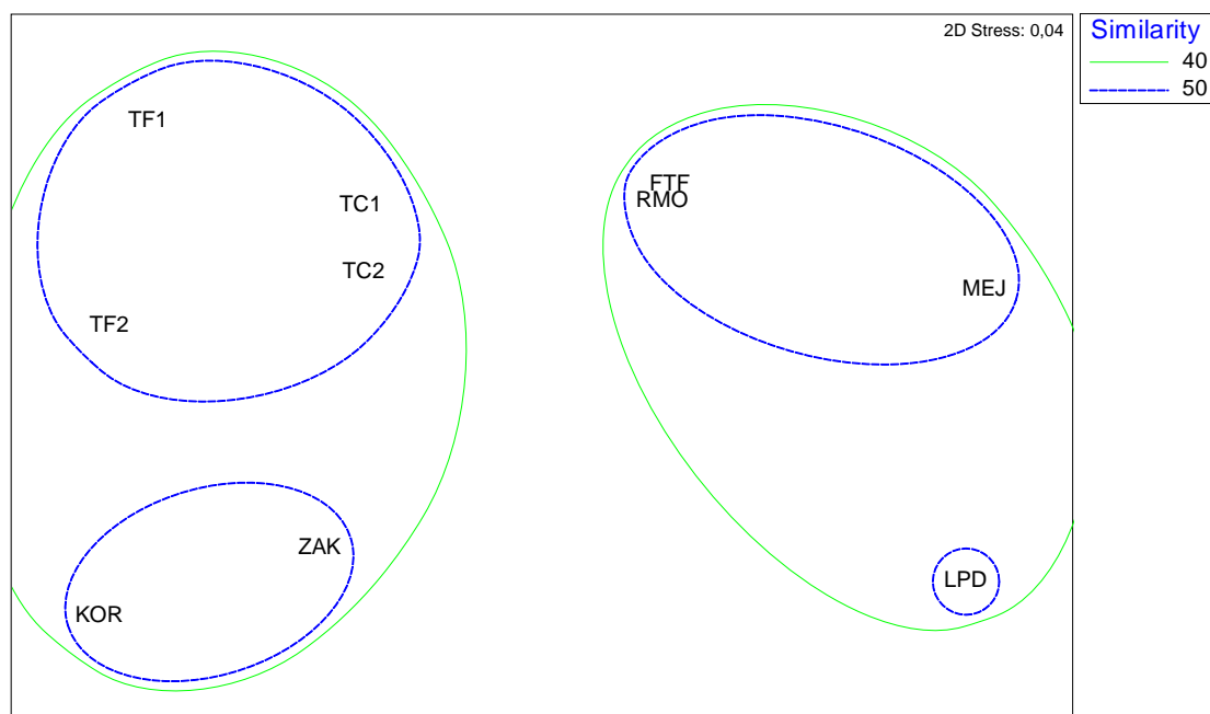
Figure 9. nMDS plot showing similarity among stations, based on presence-absence data.
