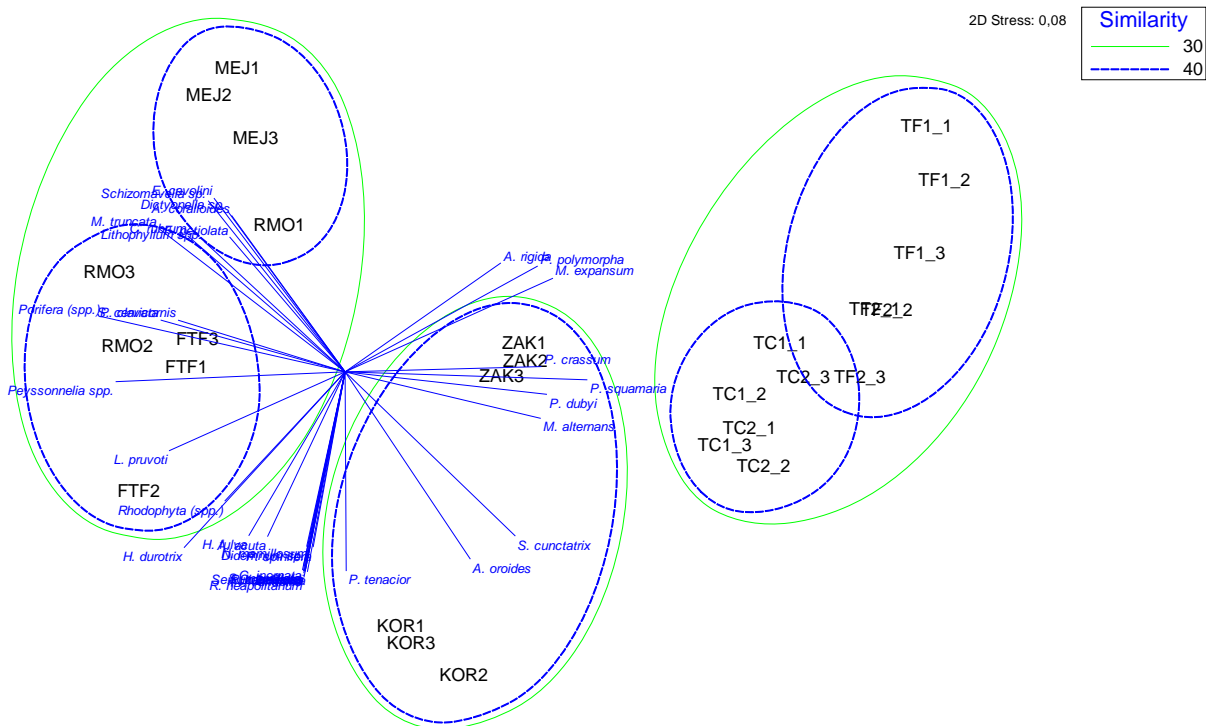
Figure 23. nMDS plot of samples based on species point/coverage data and the correlation of important species ( r > 0.6 ) with MDS axes, represented by superimposed vectors. The similarity among stations was estimated using the Bray-Curtis similarity index and was secondarily over-imposed on the nMDS plot.
