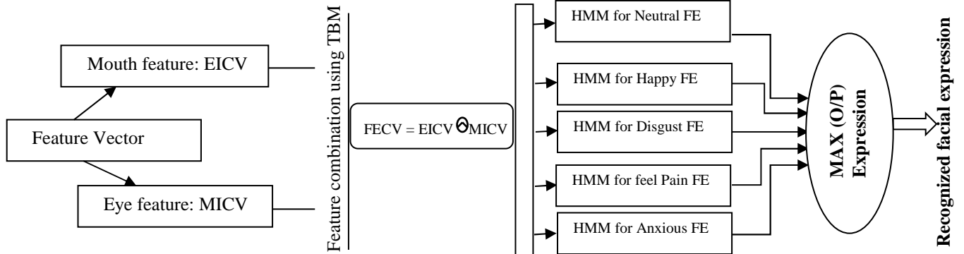
Figure 4: An illustration for Ev-HMM architecture to recognize facial expressions
