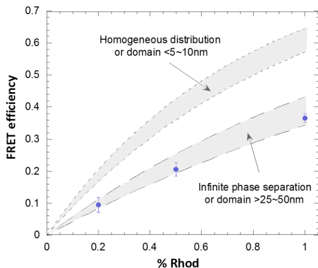
Figure 8. FRET efficiencies vs. content (mol %) of lipid-labeled acceptor for PEO 8 - b -PDMS 22 - b -PEO 8 /DPPC (79/21 w/w%) mixtures at 46 °C. Theoretical expectation for the case of homogenous distribution and infinite phase separation taking into account experimental uncertainty in the area/polymer chain determination are delimited by shaded areas.
