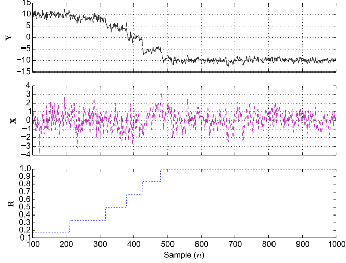
Fig. 5. Trajectories of simulated CGOMFSM (\mathbf{X}_1^N, \mathbf{Y}_1^N, \mathbf{R}_1^N) .
