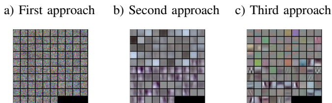
Fig. 6. Conv1 filters after 135 000 iterations.
