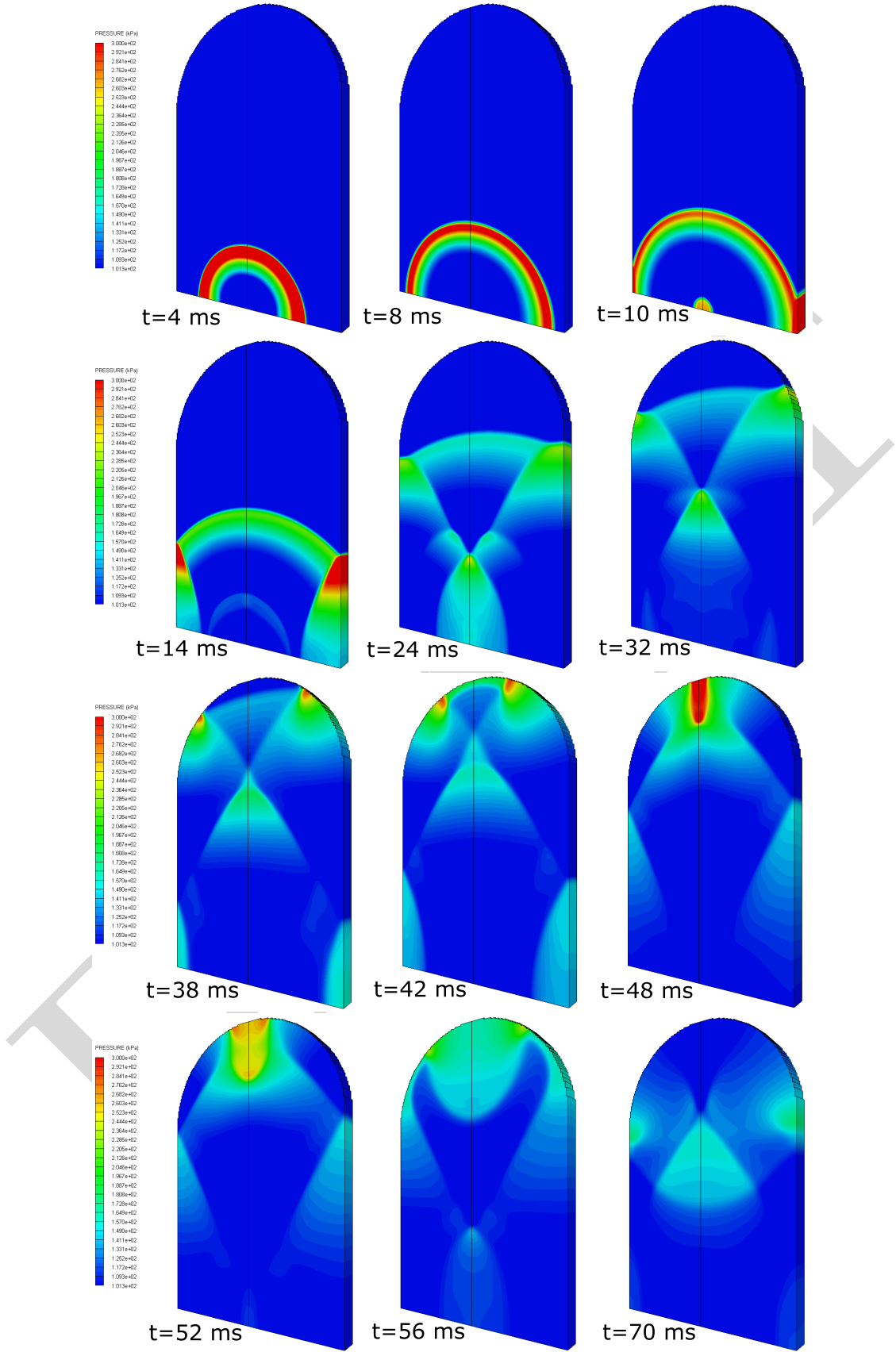
Figure 14: Evolution of the shock-wave as predicted by JWL.
