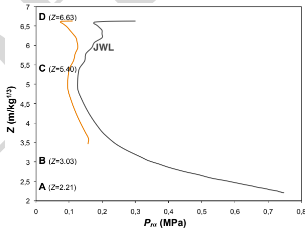
Figure 16: Comparison of P_{ra} as obtained by JWL for the two cases of complete vertical walls (black curve) and of openings until the height of 7 m (orange curve).
