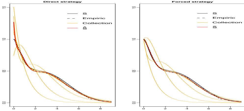
FIGURE 1. Direct observations. Survival function estimation. X \sim M\Gamma , n = 100 . In dotted bold S , in plain orange (light grey) \hat{S}_{\tilde{m}} on the left and \tilde{S}_{\tilde{m}} on the right, in plain bold red (black) \hat{S}_{m_{\max}} on the left and \tilde{S}_{m_{\max}} on the right.
