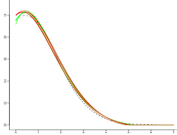
FIGURE 2. Additive model. Survival function estimation. X \sim \chi^2 , n = 200 . In dotted bold f , in plain green (light grey) 6 final estimators \hat{S}_{\hat{m}} , in plain red (black) 6 final estimators \tilde{S}_{\tilde{m}} .
