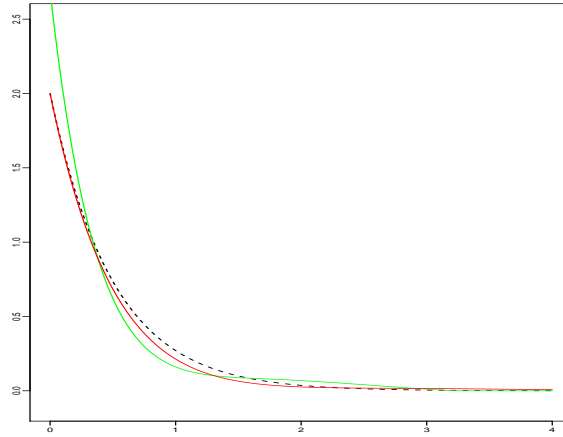
FIGURE 3. Multiplicative model. Density estimation. X \sim \mathcal{E}(2) , n = 100 . In dotted bold f , in plain green (light grey) \hat{f}_{\hat{m}} , in plain red (black) \tilde{f}_{\tilde{m}} .
