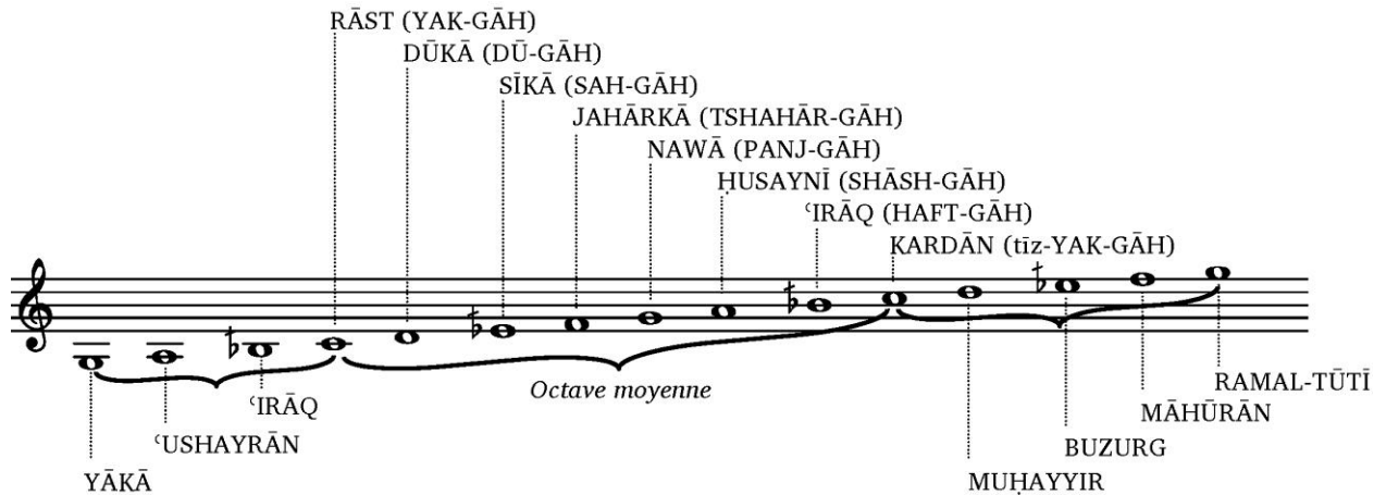
FHT 21 The General bi-octavial scale of Arabian music according to Erlanger, with the “modern” names of the degrees 1050 .
