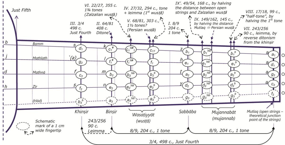
FHT 17 (Al-) Fārābī’s theoretical division of the fingerboard of the ‘ūd 1046 .
