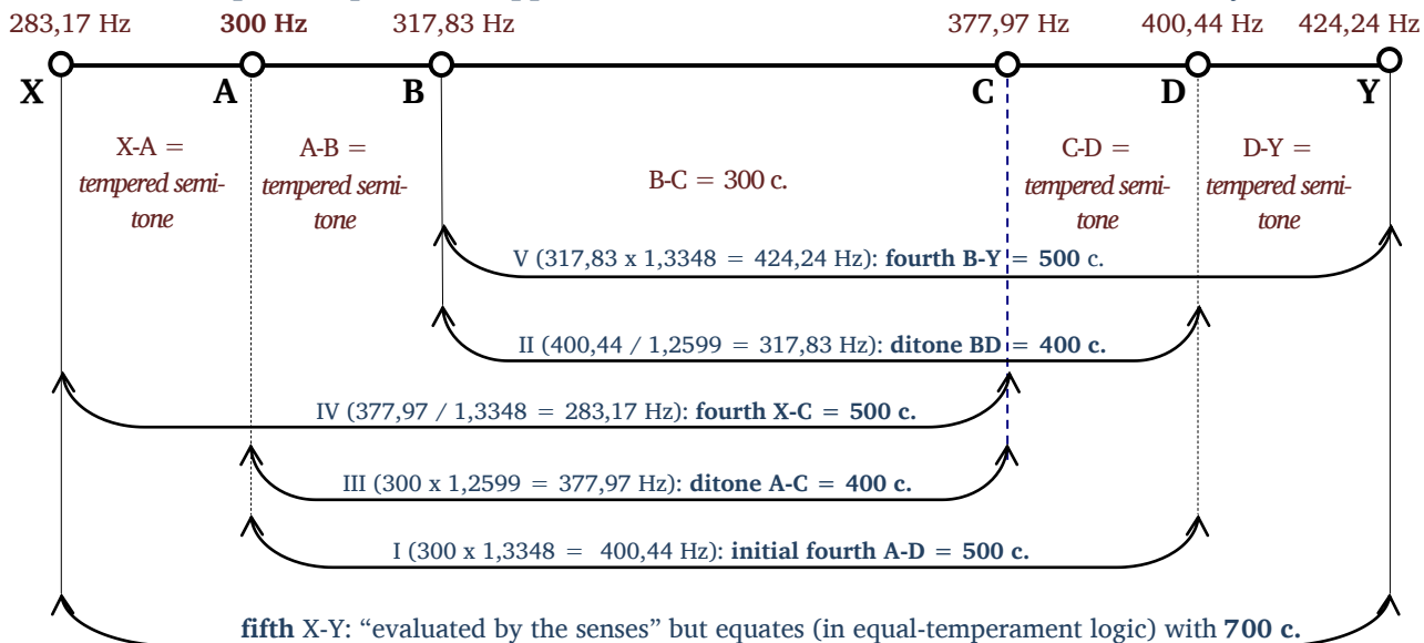
FHT 36 Applying Equal-temperament logic for the determination of the value of the half-tone – all intervals are tempered on an equal-semitone basis and match their equal-tempered values (see Slide No. 12).
