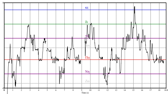
Fig. 84 Tonometric analysis of an excerpt of Kyrie Ekekraxa (Byzantios-Murr) in the diatonic Byzantine scale as performed by Fr. Nicolas Malek 790 .
