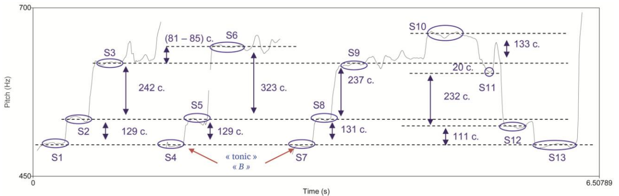
FHT 8 3 examples of hijaz by Kudsi Erguner ( na'y ): the 2 nd example is, according to the (Turkish) performer, “to be avoided”. Recorded in Paris at the performer’s home, September 2005; tonometric analysis with Praat – Slide No. 18 1040 .
