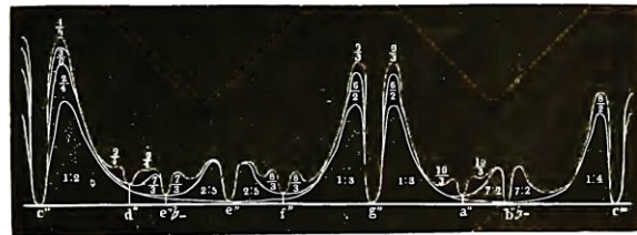
FHT 56 Two diagrams by Helmholtz showing “roughness” curves in relation with a fundamental sound 1166 .
