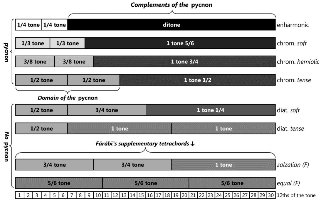
FHT 43 Aristoxenos' typical genera (in tetrachordal representation, the six above), with intervals expressed in fractions of the (equal-tempered) tone on a grid in multiples of the twelfth of the tone (or Byzantine minutes – 72-ET), and (al-) Fārābī's additions (the two tetrachords below); the soft diatonic is the prototype of the Arabian original hijāz (3/4 tones, 5/4 tones and 1/2 tone), with however a different disposition of the intervals inside the tetrachord 1148 .
