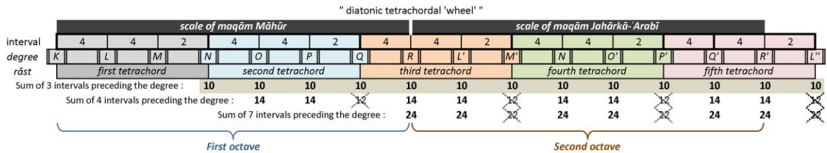
FHT 68 Ditone bi-octavial tetrachordal "wheel" 1266 .
