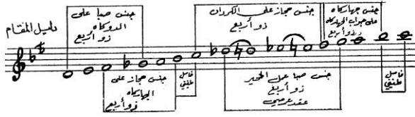
Fig. 42 (Al-) Ḥilū's notation of maqām Ṣabāʾ 's ascending scale, with a tetrachordal jins hijāz in lieu of a pentachordal hijāz based on f 377 .
