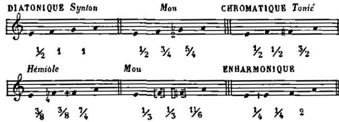
FHT 2 Weil and Reinach's notation of Aristoxenos' typical tetrachords 1034 (as for most representations, this one is chosen on e to minimize the number of accidentals).
