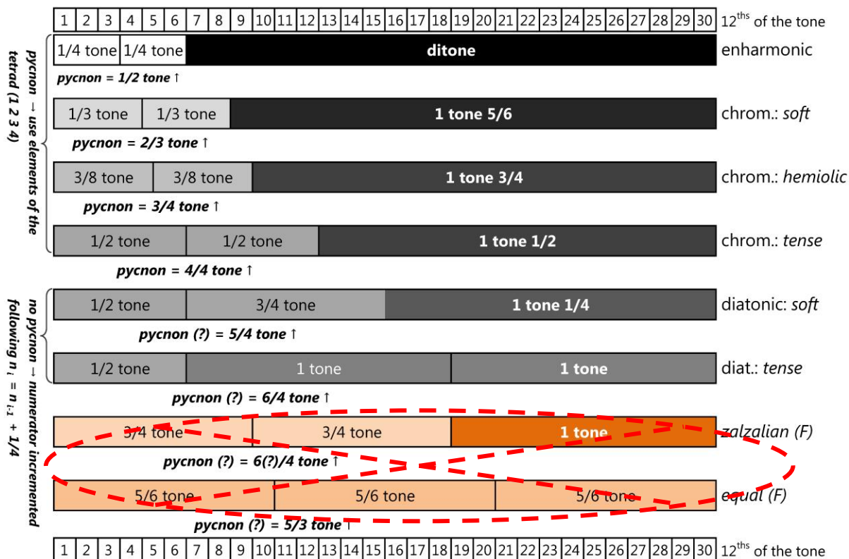
FHT 49 The “equal-intervals” hypothesis for Fārābī’s developments of Aristoxenos’ genera not fitting the Pythagorean model immanent in Aristoxenos’ exposé.
