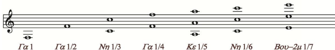
FHT 53 The first seven harmonics and their correspondence with Byzantine degrees of the scale according to Chrysanthos 1163 : notation of the partials pitch is approximate and provided exclusively as a reminder.
