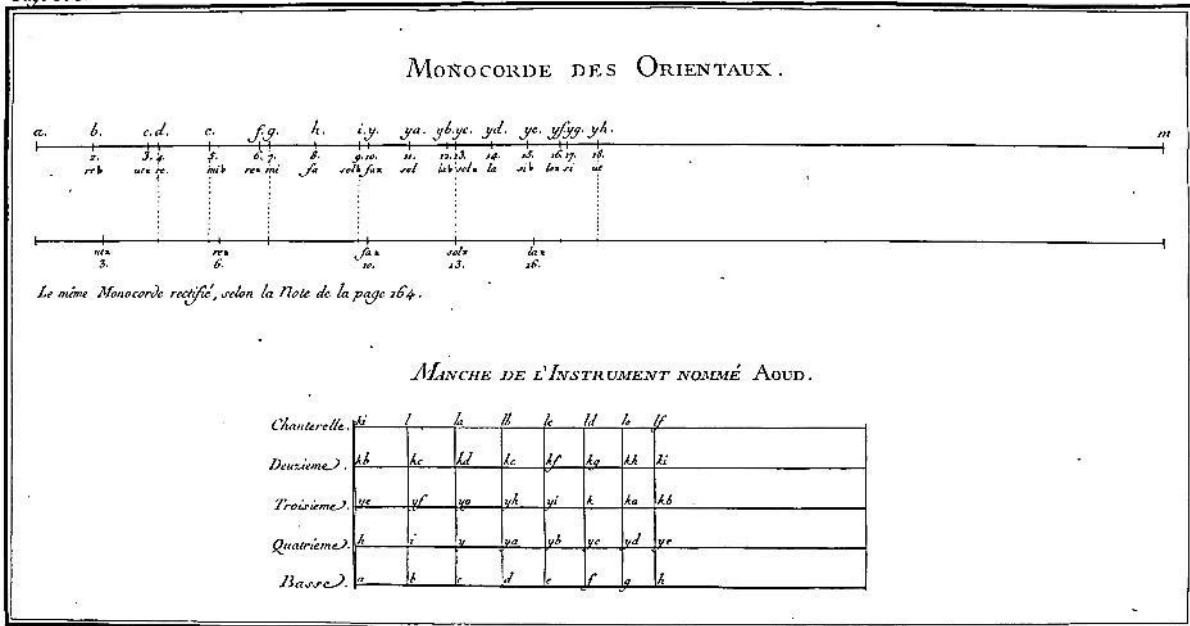
FHT 18 Division of the neck of the ‘ūd with presumed tablature and alphabetical notation (below), and correspondences (above) with the ditonic scale according to [Laborde (de), 1780a, v. 1, p. 163]; this (Systematist) division is attributed to the “Turks and the Persians” 1047 .
