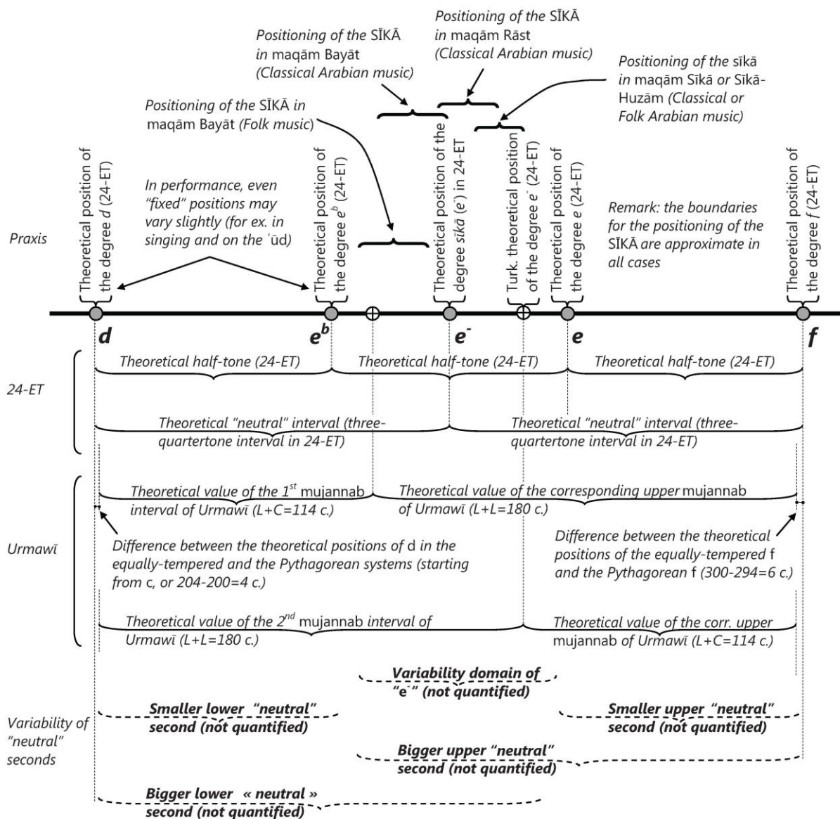
FHT 6 Theoretical and practical models for the degree SĪKĀ ( e ) in maqām music 1038 .
