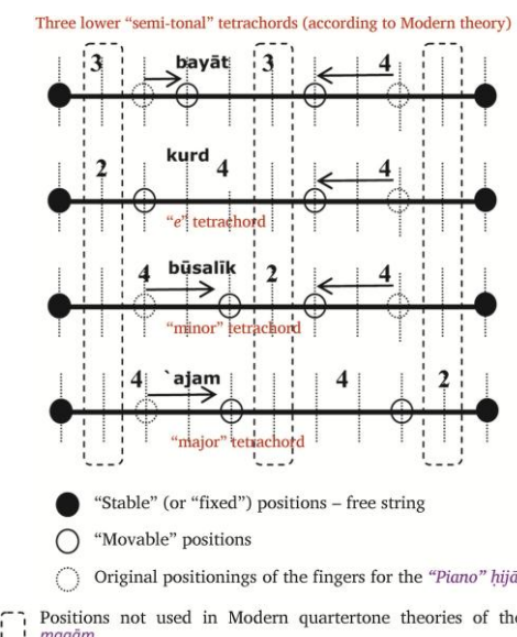
Fig. 20 The tetrachords in generic Arabian theories and the positioning of the internal notes on a schematic equal-length basis – Part II.
