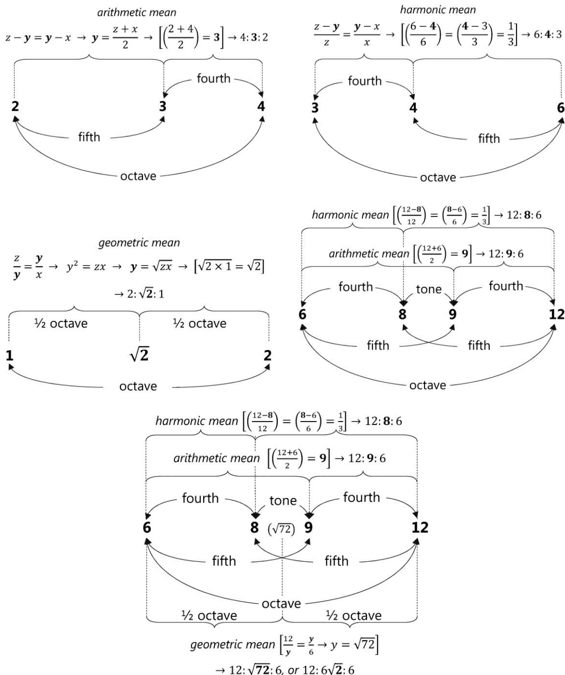
FHT 1 The three main means (adapted and translated from [Beyhom, 2010c]) 1033 .
