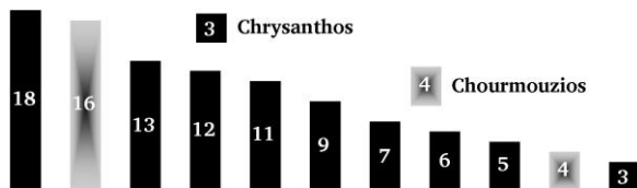
Fig. 68 Intervals of second explicitly used in Chrysanthos’ and Chourmouziotis’ “systems” and polychords 636 .
