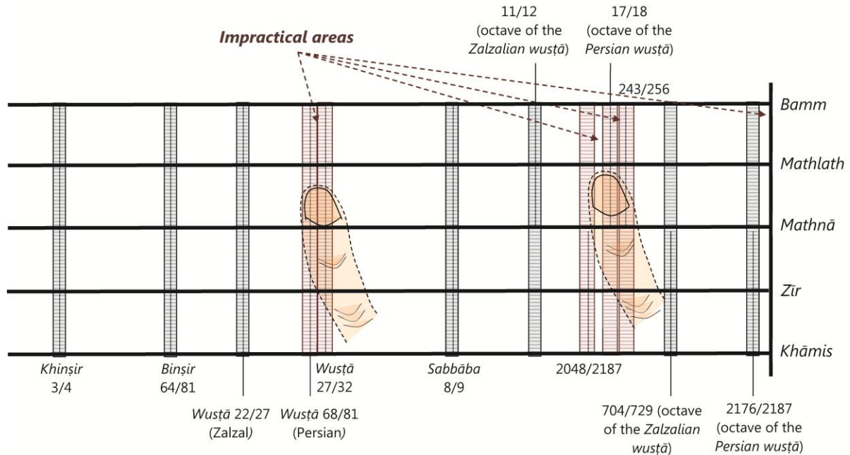
FHT 31 In the case of effective “fretting” (tying of strings around the neck of the ‘ūd) – here for the meshing of (al-) Fārābī, medium double-ties 1mm thick would nearly overlap on the fingerboard, making it impossible to play in some areas; using (al-) Kindī’s ties would lead, in the case of Fārābī’s meshing, to a clear impossibility of performance 1061 (see the following figure).
