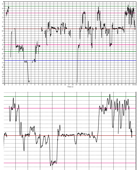
Fig. 21 Pitch analysis of the performance by Sheikh 'Ali Maḥmūd of Yā Nasīma-ṣ-Ṣabā (above), with the detailed analysis of the ḥijāz jins below 143 .
