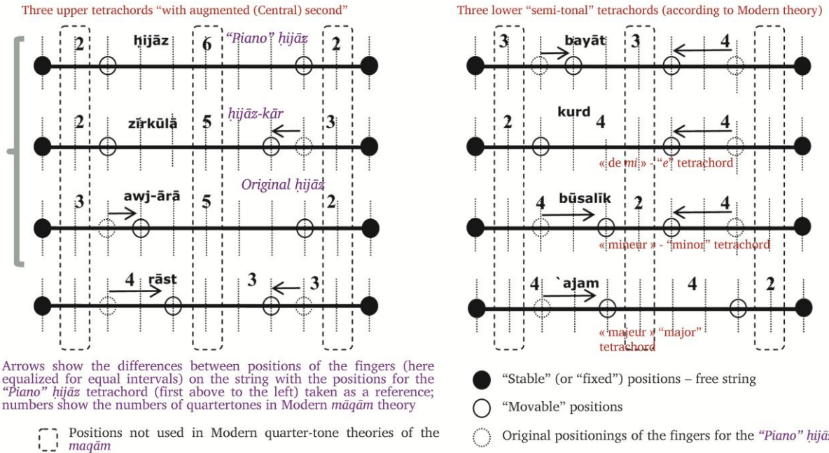
FHT 7 Typical genera (as tetrachords in their typical formulation in a given repertoire) in Arabian maqam music – performed by Hamdi Makhoul in the accompanying power point demo (Slide No. 17); names of tetrachords in black 1039 are older names found in various literature in Arabic, with updated denominations (see for example [Beyhom, 2014a]) in purple – this is the original sketch of Fig. 32.
