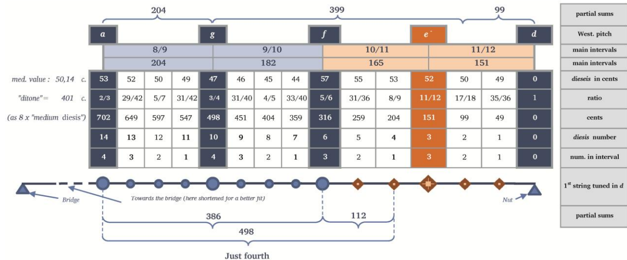
FHT 42 Alternative reasonings for the “24-dieseis” division based on a dual 12-parts main division of the string and divisions in 3 dieseis of the first 2 (ascending) “tones” and 4 “dieseis” for the last two tones; all divisions are equal-divisions of the string(s), with each of the 8/9, 9/10, 10/11 and 11/12 “tones” subdivided in either 3 (for the tones with ratios 11/12 and 10/11) or 4 (for the tones with ratios 10/9 and 9/8) equal-length parts 1122 .
