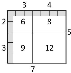
Fig. 3 Obtaining the tetraktys 6 8 9 12 on the basis of the tetrad 44 .
