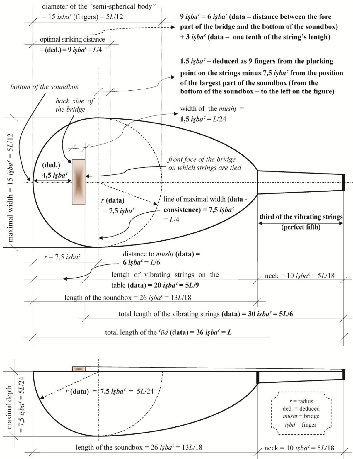
FHT 28 (Al-) Kindi's description of the 'ūd, in "finger ( ishba c - aṣābi )" thicknesses" measurements, and deduced (calculated) proportions 1059 . The same procedure is used for the "Harmonic mesh" shown on the next figure.
