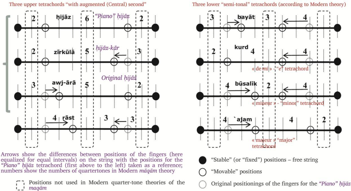
FHT 7 Typical genera (as tetrachords in their typical formulation in a given repertoire) in Arabian maqām music – performed by Hamdi Makhlof in the accompanying power point demo (Slide No. 17); names of tetrachords in black 1039 are older names found in various literature in Arabic, with updated denominations (see for example [Beyhom, 2014a]) in purple – this is the original sketch of Fig. 32.
