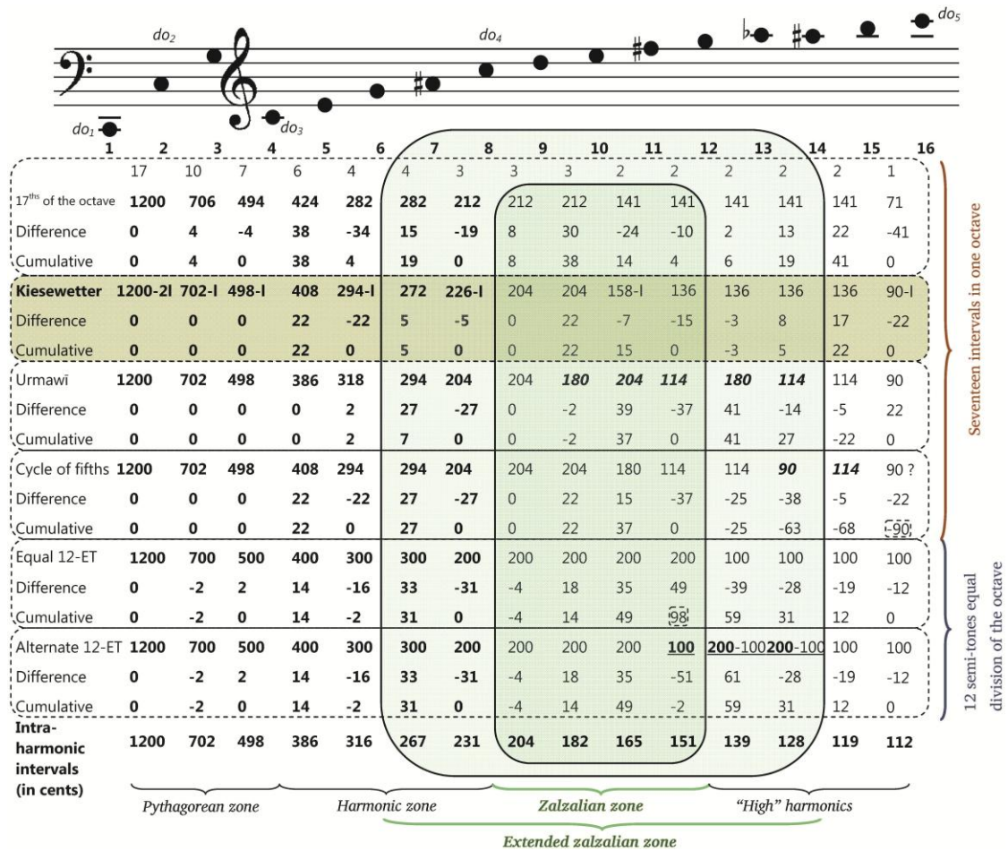
FHT 59 (Taken from the author’s habilitation thesis [Beyhom, 2010b]): Harmonic progression notated on the basis of a 17 th Equal-intervals division or 17-ET ( # shifts by one elementary interval – see [Beyhom, 2010a; 2013], here a 17 th of the octave – approx.. 71 cents, b lowers by the same value) with six sets of rows for 6 different divisions of the octave (and notations) 1169 .
