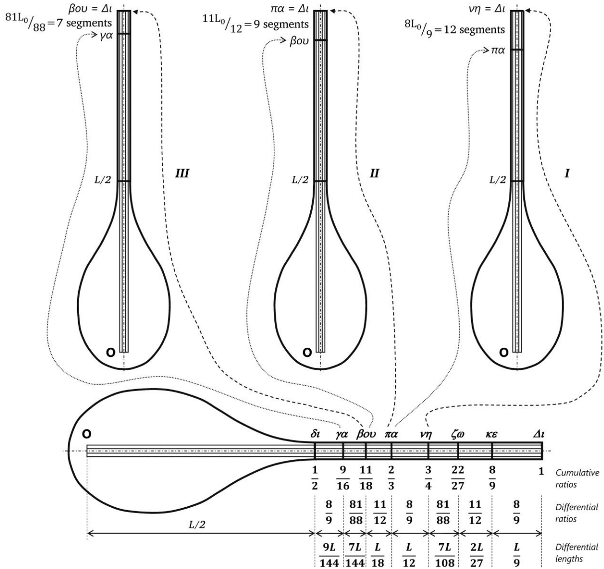
FHT 24 The procedure of the two tunbūr (s) as explained by Chrysanthos 1051 : “One could experience this truth this way: One takes two pandourides , one of which is not fretted, the other being fretted with the tones of our music as precisely as possible. He then makes the buzz [lowest note – of the free string] of the unfretted pandouris symphonous with the \nu\eta of the fretted one and supposes that this buzz is the \delta\iota . He then plays on the fretted pandouris the \pi\alpha and looks for its symphony on the unfretted pandouris . Wherever he finds it, he writes the \kappa\epsilon . He then divides this newly found interval \delta\iota\ \kappa\epsilon into twelve sections 1052 . Then he makes the same buzz symphon[i]ous with the \pi\alpha and plays the \beta\upsilon\upsilon , then he looks for its symphony and wherever he finds it, he writes the \zeta\omega 1053 . He then makes the same buzz again symphon[i]ous with the \beta\upsilon\upsilon , plays the \gamma\alpha , looks for its symphony and wherever he finds it, he writes the \nu\eta 1054 . Then he observes the newly written notes and finds out that the \kappa\epsilon is written on the 12, the \beta\upsilon\upsilon on the 9 and the \gamma\alpha on the 7 1055 .
