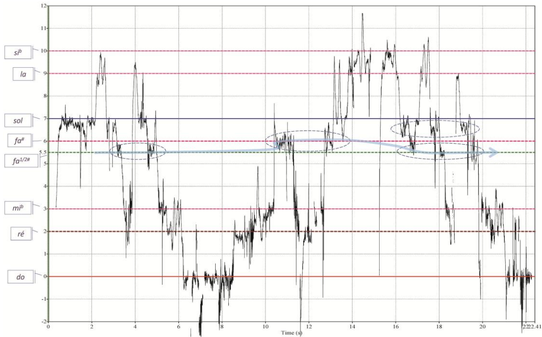
FHT 11 Tonometric analysis with Praat of the beginning of the song Ḥawwīl yā Ghannām performed by Lebanese singer Najāḥ Salām (1947?), showing the displacement of the “lichanos” between fa^{1/2\#} ( fa^{1/2\#} ) and fa^\# ( fa^\# ) depending on the melodic movement (ascending, descending, stopping, etc.) 1043 – see Slides Nos. 22-23.
