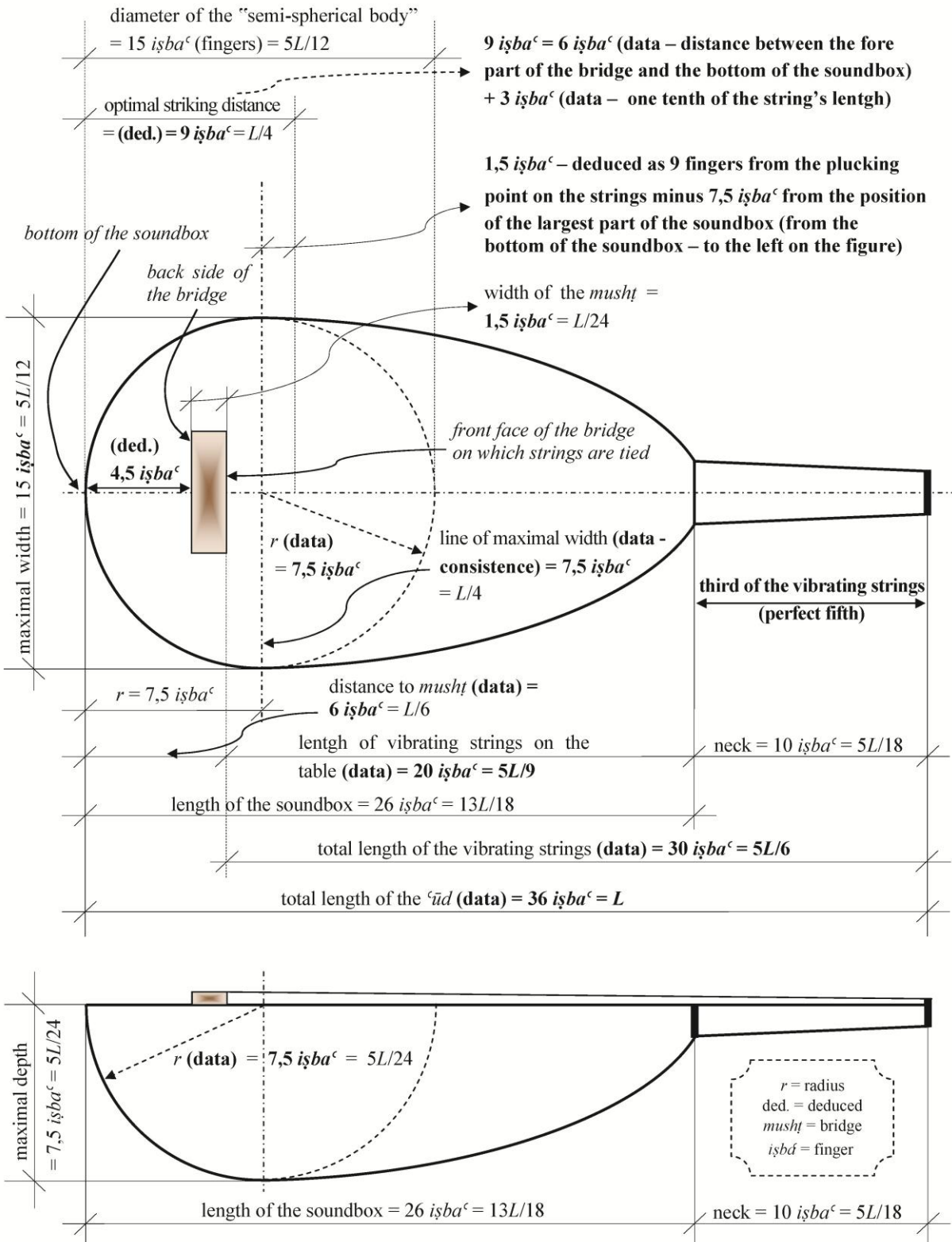
FHT 28 (Al-) Kindi's description of the 'ud, in "finger ( ishba - aṣābī )" thicknesses" measurements, and deduced (calculated) proportions 1052 . The same procedure is used for the "Harmonic mesh" shown on the next figure.
