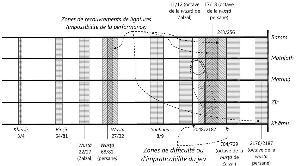
FHT 32 Figure 129 from [Beyhom, 2010c, v. 1, p. 358] showing the overlapping “frets” in case ties are notted around the neck of the ‘ūd following Kindī’s indications; note that Kindī was the only theoretician who described the “physical” ties (most probably for beginners) giving decreasing proportions (thicknesses) from the nut and in the direction of the bridge – the number of ties he described was however limited to four.
