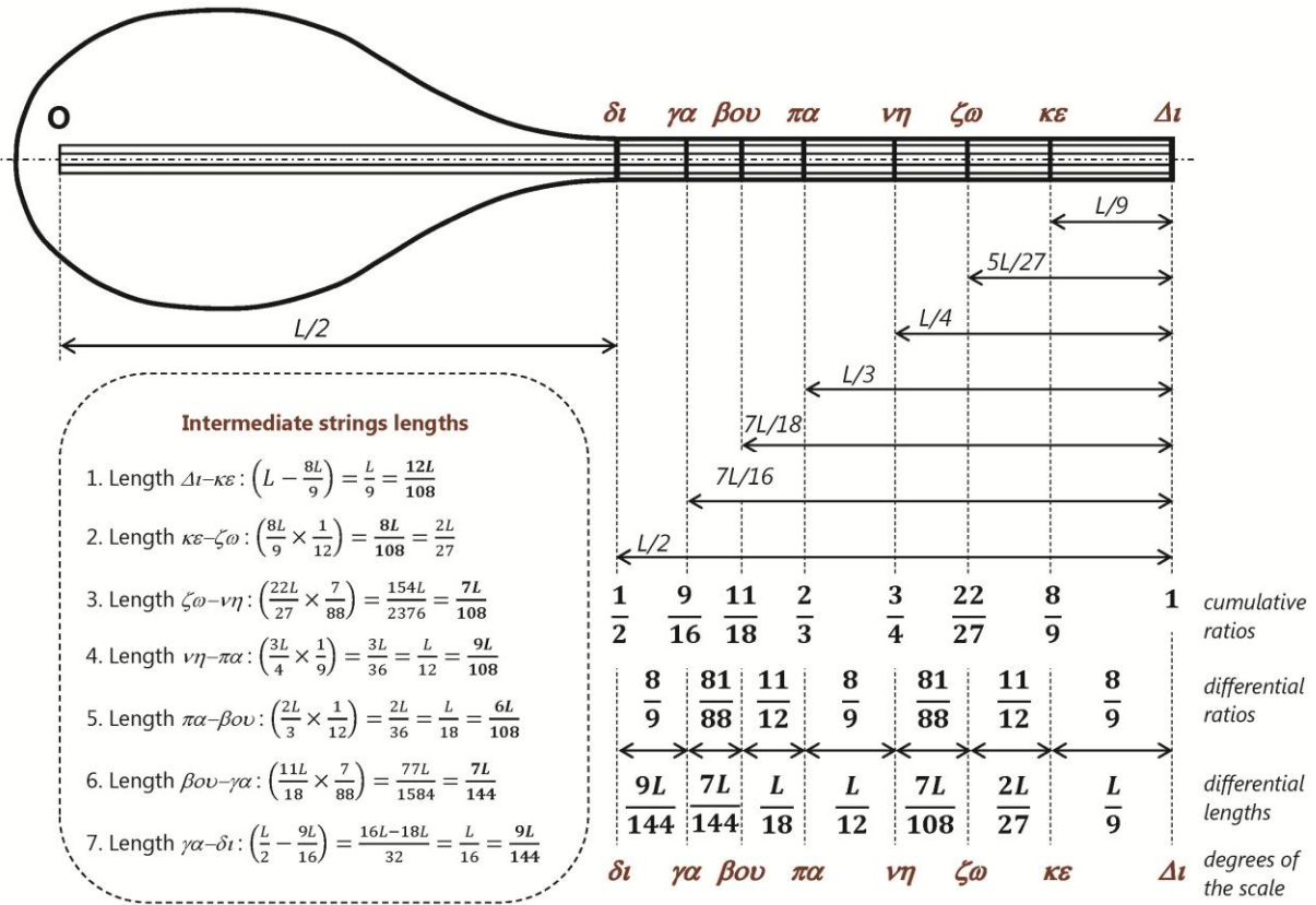
FHT 22 Chrysanthos Madytos' detailed division of the strings on the neck of the tunbūr (translated and adapted from [Beyhom, 2015b, p. 185]).
