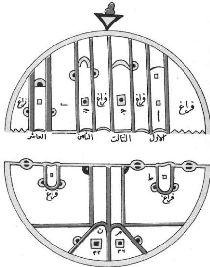
FHT 60 A schematic representation of the "Automatic Organ" by the Banū Mūsā (9 th century) 1180 .
